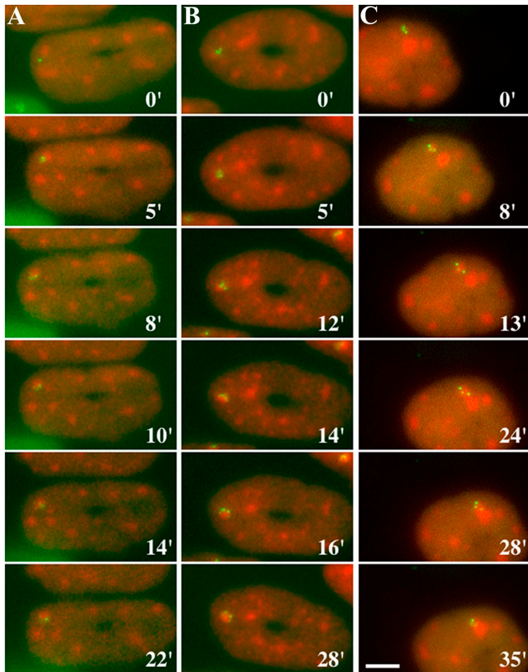
Figure 6. Live imaging shows three possible transgene/speckle dynamic events during heat shock. (A) Long-range movement of Hsp70 BAC transgenes (green) toward a ASF/SF2 speckle (red) occurred within a 5-min heat shock period (Video 1). (B) Enlargement of preexisting speckle together with decondensation and increased association and encircling of BAC transgenes around speckle exterior (Video 2). (C) Nucleation of a new ASF/SF2 speckle adjacent to the Hsp70 BAC transgenes several minutes after heat shock; newly nucleated speckle then merges with preexisting adjacent speckle forming a larger speckle (Video 3). Bar, 5 \mu m.
