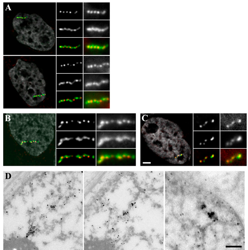
Figure 3. No evidence for extended looping of BAC sequences from a linear backbone. (A–C) 3D DNA FISH shows co-linear signals from the Lac operator (red) and BAC (green) probes. DNA is stained by DAPI (gray). (A) DHFR D10 cells. (B) DHFR-110-5-E4 cell with lac operator repeats inserted into the DHFR gene fifth intron. (C) Hsp70_5 cell 30 min after heat shock. Middle columns (deconvolved data) and right columns (raw data) show 2x enlarged views (Bars, 2 \mu m). (D) EM of DHFR D10 clone by in vivo immunogold staining of EGFP-LacI shows the BAC transgenes are compacted indistinguishable from surrounding genomic DNA, with no obvious looping structure from the transgene backbone. Left and middle: serial sections (150 nm); right: 500-nm section (Bar, 500 nm).
