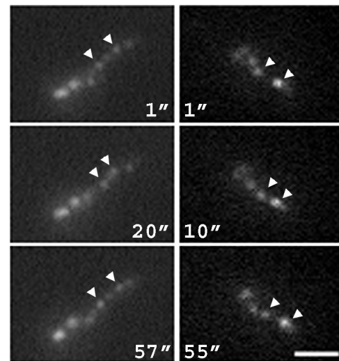
Figure 7. Rapid movement of DHFR BAC transgenes along the transgene array axis implies chromatin conformational changes over a several second time scale. Live-cell imaging of DHFR BAC B9 cell line with \sim 1 -s time intervals (Video 4). Two examples (left and right) show GFP spots moving relative to each other (arrowhead) along the direction of the BAC transgene array chromosome axis. Video 4 shows most GFP spots are in rapid motion relative to each other on a time scale far shorter than the estimated 10 min required for complete transcript synthesis, implying the absence of stable attachments of transgenes to surrounding nuclear structures during transcription. Bar, 2 \mu m.
