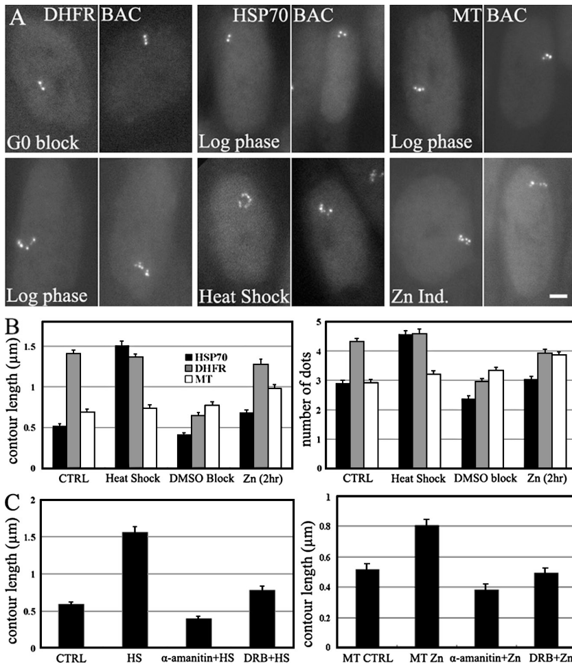
Figure 2. Large-scale chromatin decondensation accompanies gene activation. (A) GFP-lac repressor fluorescence before (top) and after (bottom) gene induction for the DHFR (O57L22), Hsp70, and MT BACs. After induction, a more extended “string of dots” is observed. Bar, 2 μm. (B) Histograms showing mean contour lengths (left) or GFP spot number (right) for each BAC cell line at normal growth conditions (CTRL) (DHFR gene induced) and after heat shock (Hsp70 genes induced), Zn addition (MT genes induced), or DMSO induced G1 arrest (DHFR repressed) (see text). Increases in contour length and spot number are specific for the induction conditions appropriate for the particular BAC transgene. (C) Histograms showing contour length under CTRL or induced conditions for Hsp70_5 and MT_1_4 cell lines with and without transcriptional inhibition. Chromatin decondensation accompanying heat shock is blocked by α-amanitin and significantly reduced by DRB (see text). (B and C) Histogram data points are based on > 100 cells (SEM error bars).
