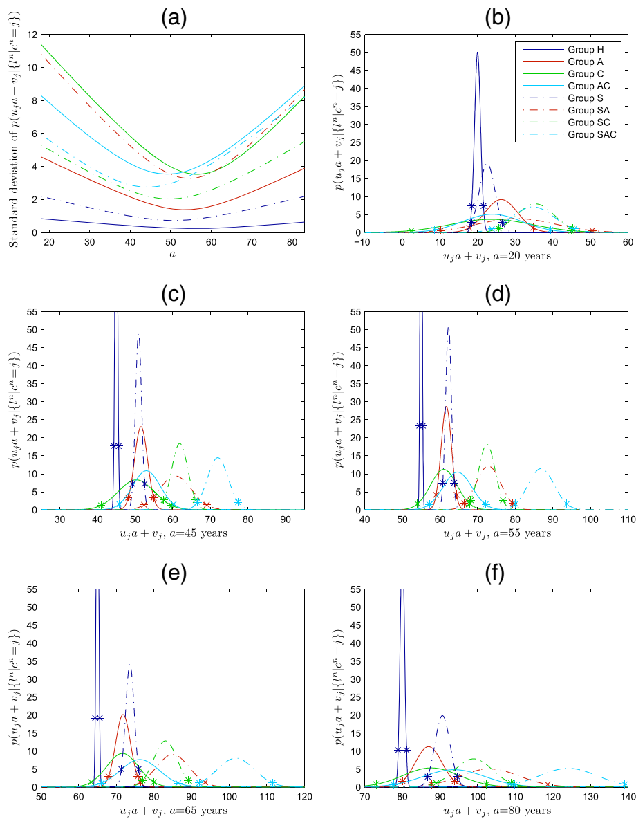
Figure 6 Posterior distributions p(u_j a + v_j | \{I^n | c^n = j\}) . (a): Standard deviations of the posterior distributions p(u_j a + v_j | \{I^n | c^n = j\}) . (b-f): Posterior distributions p(u_j a + v_j | \{I^n | c^n = j\}) for ages a = 20, 45, 55, 65 and 80 years. The length between two starts equals 2 \times 1.96 times the standard deviation. The legend in (b) is valid for all plots.
