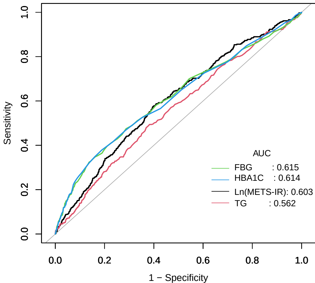
ROC curve for GDM
