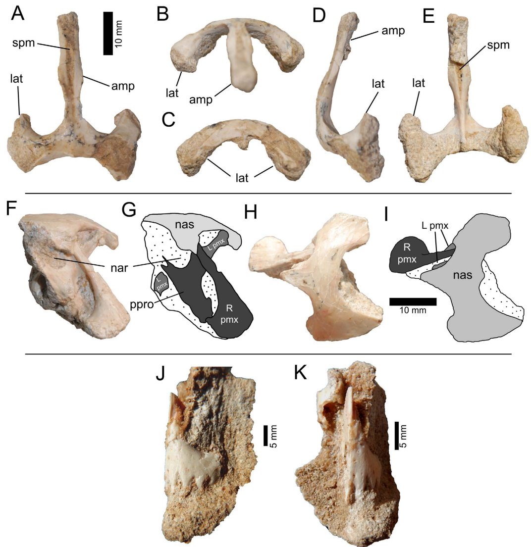
Figure 4. MPC-D 102/46, Avimimus . Fused nasals in dorsal (A), anterior (B), posterior (C), right lateral (D), and ventral (E) views. MPC-D 102/34, Avimimus . Block containing right premaxilla, maxilla and fused nasals in lateral (F,G) and dorsal (H,I) views. MPC-D 102/108, Avimimus . Block containing two nearly articulated premaxillae in left lateral (J) and anterior (K) views. Abbreviations: amp , anterior midline process; lat , lateral descending process; L pmx , left premaxilla; nar , naris; nas , nasal; ppro , posterior process of premaxilla; R pmx , right premaxilla; spm , slot in nasal for premaxilla.
