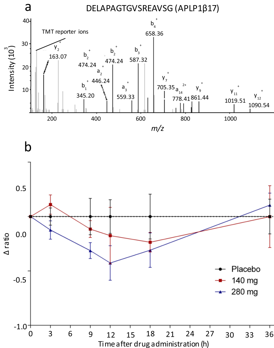
Fig. 3 APL1 \beta 17. The peptide DELAPAGTGVSR EAVSG, constituting fragment APL1 \beta 17 from amyloid-like protein 1 (APLP1). a Annotated MS2 spectrum. b Relative abundance of the peptide after semagacestat treatment. In the 280 mg dosage group the concentration of the peptide decreased to a minimum of 32 % at 12 h ( p=0.0018 ), and in the 140 mg group the minimum relative concentration was 15 % at 18 h ( p=0.078 ). Graphed data are medians with median absolute deviations
