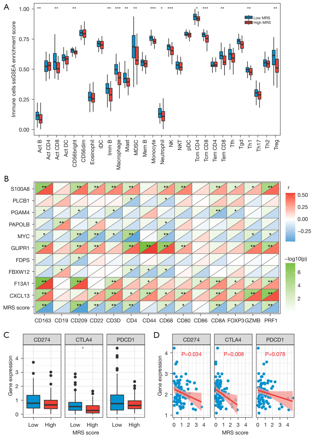
Figure 3 Correlation analysis between the MRS and the immune microenvironment. (A) Boxplot of the different immune cells in patients with different MRS. (B) Correlation between MRS genes and immune cell markers. (C) Relative expression of the immune checkpoints. (D) Correlation between the MRS score and the expression of the immune checkpoints. *, P < 0.05 ; **, P < 0.01 ; ***, P < 0.001 . ssGSEA, single sample gene set enrichment analysis; MRS, metastasis-related gene signature.
