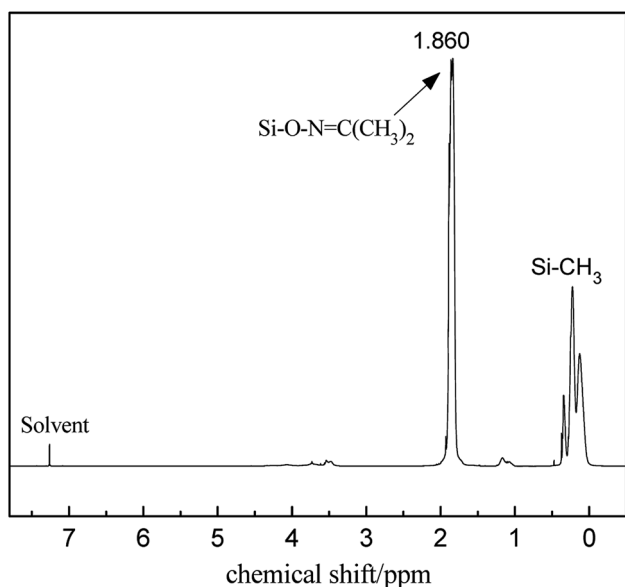
Fig. 3 1 H NMR spectrum of PMKS.
