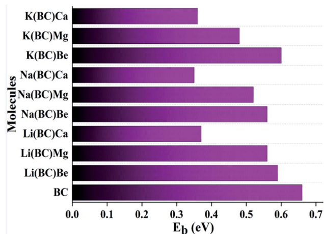
Fig. 5 Graphical representation of the binding energies of surface BC and all the newly designed molecules.
