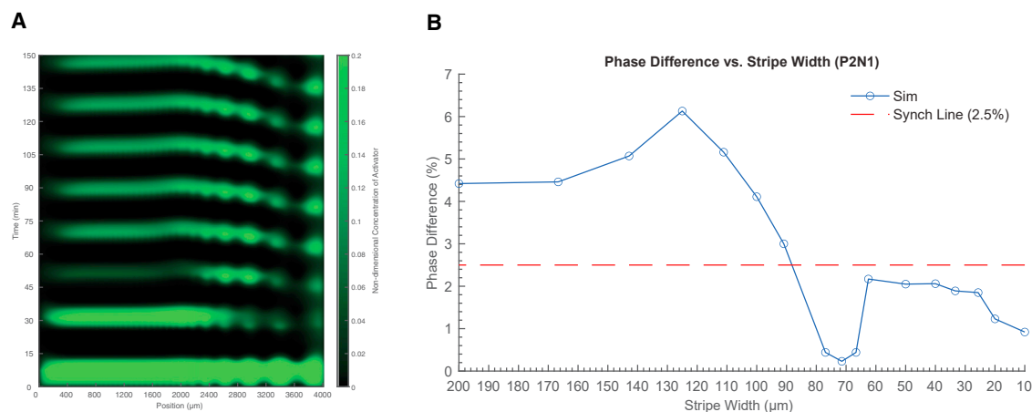
FIGURE 3 Spatial organization's influence on synchrony. (A) Kymograph of activator concentration in the P_2N_1 consortium consisting of heterogeneous stripes. The left side of the consortium consists of small-width stripes (0.56–47.06 \mu\text{m} ), and the right side of the consortium consists of large-width stripes (19.05–266.67 \mu\text{m} ). (B) Graph showing the relationship between phase difference and stripe width for the P_2N_1 consortium.
