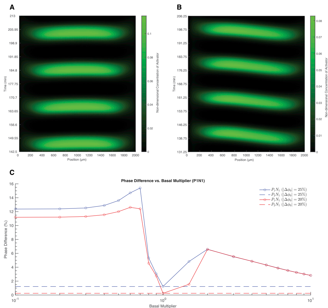
FIGURE 2 Basal production's influence on synchrony. Results of our synchronization simulations including kymograph of activator concentration during the 8th to 11th oscillations of the P_2N_1 (A) and P_1N_1 (B) consortia (basal multiplier of 0.7). (C) Graph showing the relationship between phase difference and the value of the basal multiplier for the P_1N_1 consortium at two different initial phase differences, |\Delta\phi_0| = 25\% and 20\% .
