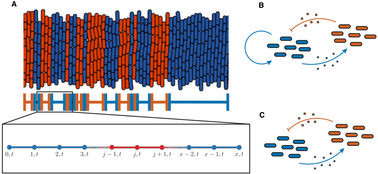
FIGURE 1 Consortial organization. (A) Micro and macro illustration of our spatial discretization that allows for the incorporation of columnar spatial patterns in the P_2N_1 and P_1N_1 consortia. For spatial points corresponding to activator segments (blue), the production terms for the repressor, \eta_{r_0} and \eta_{r_1} , are set to zero. The opposite holds in the repressor segments (orange) where the the production terms for the activator, \eta_{a_0} and \eta_{a_1} , are set to zero. Diagram of the P_2N_1 (B) and P_1N_1 (C) gene circuit topology.
