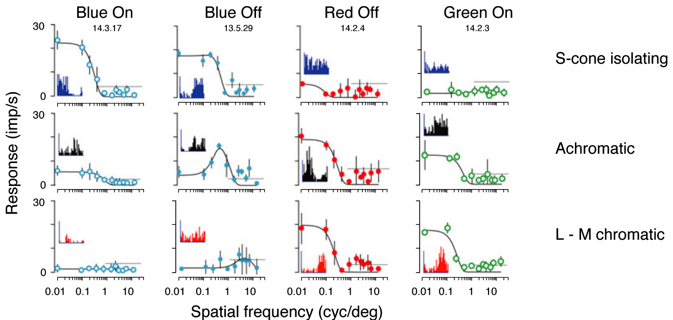
Fig. 2. Classification of LGN cells. Each column shows spatial frequency transfer functions for one cell of the indicated response type. Each row shows responses to one stimulus type. The top row shows responses to stimuli modulating only the S-cones and the second row shows responses to achromatic gratings modulating all three cone types in additive phase. The lower row shows responses to R/G (L–M) chromatic modulation. The temporal frequency of the drift was 4 Hz and the orientation was optimised for each cell. The cone contrasts for each stimulus are shown in Table 1. The insets show PSTHs made with a bin width of 10 ms from the response to a low (0.01 cycles/deg) spatial frequency condition in each panel. The phase of Blue On cell responses to achromatic stimuli could be either On or Off and, in this cell, it is Off. The abscissa is 0.25 s and the ordinate 10 impulses/s. The horizontal grey lines show the amplitude of the f_1 component of the FFT in the absence of spatial contrast.
