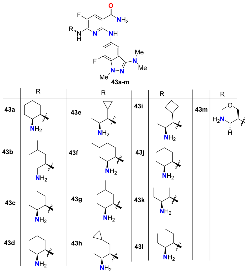
Fig. 30 Structure of 7-fluoroindazole derivatives 43a–m.
