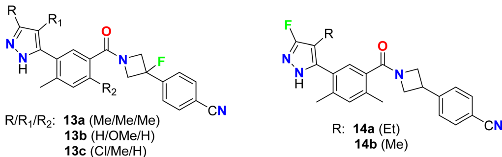
Fig. 10 Structure of 4-fluorinated azetidino-based pyrazole molecular hybrids 13 and 14.
