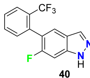
Fig. 27 Structure of 6-fluoroindazole scaffold 40.
