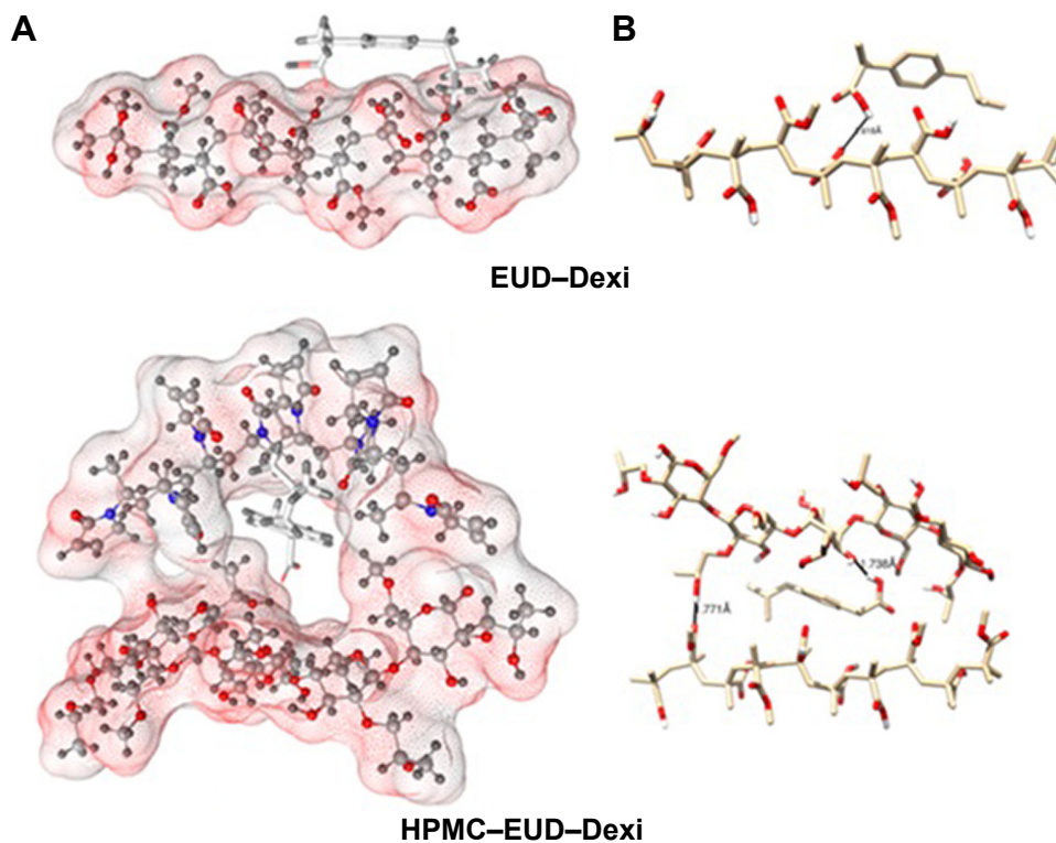
Figure 10 Interactions of EUD-Dexi (top) and HPMC-EUD-Dexi (bottom) complexes showing hydrogen bonding as black lines.
