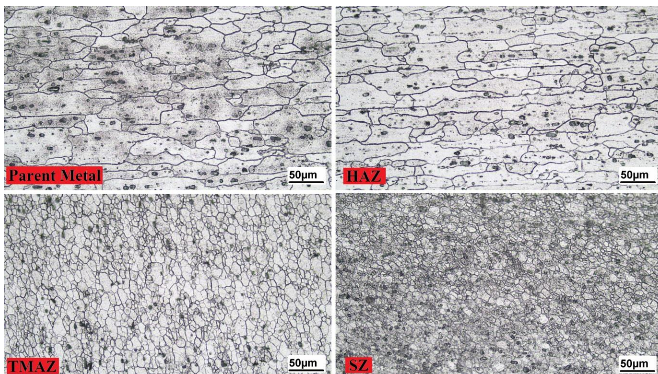
Figure 13. Microstructure of different areas of the sample welded by FSW technique.
