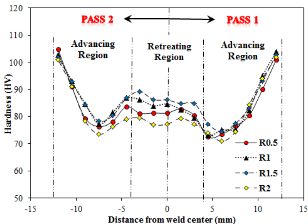
Figure 12. Hardness profiles of RP-FSW specimens with different tool offsets.
