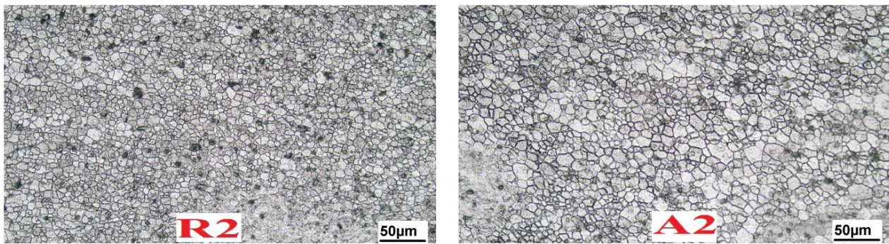
Figure 14. Distribution of SZ microstructure for welded specimens using AP-FSW and RP-FSW techniques.
