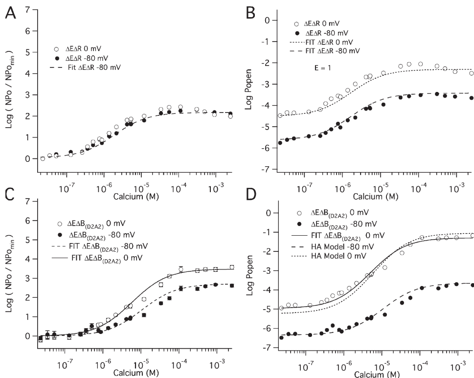
\Delta E\Delta B_{(D2A2)} is shown for patches held at 0 mV (open circles) or at -80 mV (solid circles). Each point represents the average of between 6 and 14 patches at each [Ca^{2+}] tested. The NPopen/NPopen_{min} versus Ca^{2+} relations are fitted with Eq. 6. The values of the fit parameters are: \Delta E\Delta B_{(D2A2)} : -80 mV, K_O = 4.9 \mu M and K_C = 23.2 \mu M ; \Delta E\Delta B_{(D2A2)} : 0 mV, K_O = 2.1 \mu M and K_C = 15.6 \mu M . (D) The mean log Popen versus [Ca^{2+}] relation for mutant \Delta E\Delta B_{(D2A2)} at both 0 and -80 mV. First, the 0 mV data were fitted by Eq. 14 to yield the values: K_O = 2.1 \mu M and K_C = 15.8 \mu M . The data were also fitted with the HA model. The parameters were held as follows: K_O = 4.9 \mu M , K_C = 23.2 \mu M , L_O = 1.2 \times 10^{-6} , z_L = 0.41 e , V_{hc} = 151 mV, V_{ho} = 27 mV, z_j = 0.58 e , and E = 6.03 .
