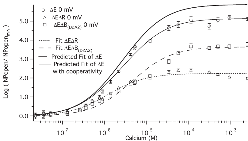
Figure 10. The two binding sites are less than additive at 0 mV. The mean log ratio of NPopen at 0 mV in the presence and absence of Ca^{2+} for mutants \Delta E (open circles), \Delta E\Delta R (open triangles), and \Delta E\Delta B_{(D2A2)} (open squares) are plotted versus [Ca^{2+}] . Each point represents the average of between 6 and 14 patches at each [Ca^{2+}] tested. Various fits of \log(NPopen/NPopen_{min}) are superimposed on the data. The fit of \Delta E\Delta R (short dashed line) with Eq. 6 yielded values of K_O = 0.63 \mu M and K_C = 2.28 \mu M . The fit of \Delta E\Delta B_{(D2A2)} (long dashed curve) yielded values of K_O = 1.56 \mu M and K_C = 12.7 \mu M . Using the same equation, we simulated the \log(NPopen/NPopen_{min}) versus Ca^{2+} relation (dark solid line) predicted by the affinities determined for each site in isolation. The parameters of the fit were: K_{O1} = 0.63 \mu M , K_{C1} = 2.28 \mu M , K_{O2} = 1.56 \mu M , and K_{C2} = 12.7 \mu M . Also
