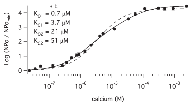
Figure 3. The \text{Ca}^{2+} binding affinity of mutant \Delta\text{E} at -80 mV. The mean log ratio of NPopo in the presence and absence of \text{Ca}^{2+} determined from the data shown in Fig. 2. \text{Log}(\text{NPopo} / \text{NPopo}_{\text{min}}) spans the entire [\text{Ca}^{2+}] range and is fit (solid line) by Eq. 5 yielding values of K_{01} = 0.7 \mu\text{M} , K_{C1} = 3.7 \mu\text{M} , K_{02} = 21 \mu\text{M} , and K_{C2} = 51 \mu\text{M} . Also shown is the fit (dashed line) assuming both types of binding sites have the same affinity for \text{Ca}^{2+} ( K_0 = 1.9 \mu\text{M} and K_C = 6.4 \mu\text{M} ). Error bars represent SEM.
