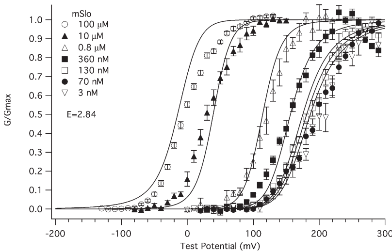
Figure 11. A modified HA model can explain the effect of Ca^{2+} on the steady-state gating properties of the BK_{Ca} channel. Shown are series of mSlo1 \alpha G-V relations determined at the following [Ca^{2+}] : 0.003, 0.070, 0.130, 0.360, 0.8, 10, and 100 \mu M and fit simultaneously with the modified model that includes two types of Ca^{2+} binding sites, one type interacts with the voltage sensor, and the other type is independent. The data are the same as shown in Fig. 8. The parameters were held as follows: K_{O1} = 0.88 \mu M, K_{C1} = 3.18 \mu M, K_{O2} = 4.88 \mu M, K_{C2} = 23.2 \mu M, L_O = 2.2 \times 10^{-6} , z_L = 0.41 e , V_{hc} = 151 mV, V_{ho} = 27 mV, and z_j = 0.58 e . The value of E coupling voltage sensor activation and Ca^{2+} binding at one type of site was allowed to vary. Shown is the best fit obtained. The value of E was calculated to be 2.84 \pm 0.13 .
