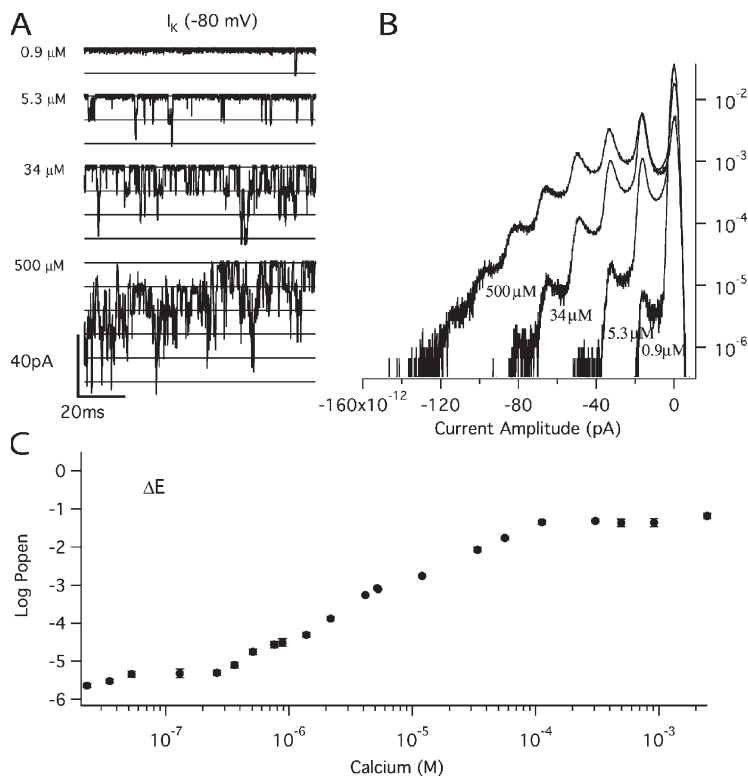
Figure 2. The \text{Ca}^{2+} dependence of Popen for mutant \Delta\text{E} . (A) Inward potassium currents recorded at -80 mV and filtered at 10 kHz from a macropatch exposed to the indicated [\text{Ca}^{2+}] demonstrate that Popen increases in a \text{Ca}^{2+} -dependent manner when voltage is constant. The corresponding all-points amplitude histograms are plotted in B on a semi-log scale and were constructed from 30-s recordings at each [\text{Ca}^{2+}] . The dose-response relation for the effect of \text{Ca}^{2+} on Popen at negative voltage ( -80 mV) is shown in C. For determination of Popen see Materials and methods. Each point represents the average of between 7 and 17 patches at each \text{Ca}^{2+} concentration tested. Error bars represent SEM.
