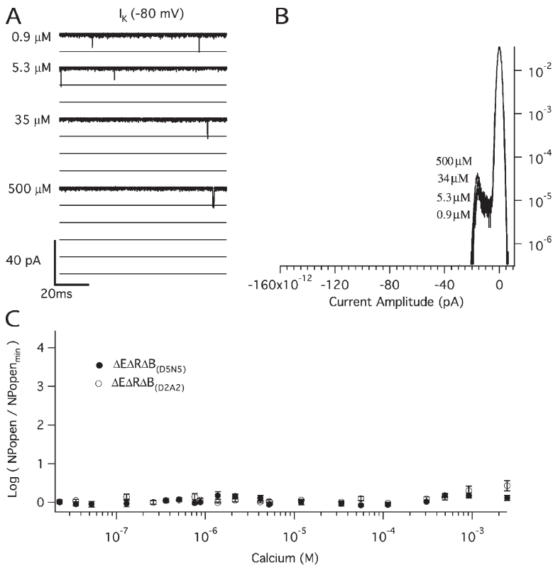
Figure 4. Mutation of all three types of \text{Ca}^{2+} binding sites eliminates the \text{Ca}^{2+} dependence of Popen . (A) Inward \text{K}^+ currents recorded for mutant \Delta E\Delta R\Delta B_{(D5N5)} at -80 mV and filtered at 10 kHz from a macropatch in the indicated [\text{Ca}^{2+}] demonstrate that Popen does not increase in a \text{Ca}^{2+} -dependent manner when voltage is constant. The corresponding all-points amplitude histograms are plotted in B on a semi-log scale and were constructed from 30-s recordings. (C) Dose-response relations for the effect of \text{Ca}^{2+} on Popen at negative voltage ( -80 mV) obtained by plotting the mean log ratio of NPopen in the presence and absence of \text{Ca}^{2+} . For both mutant \Delta E\Delta R\Delta B_{(D5N5)} (filled circles) and mutant \Delta E\Delta R\Delta B_{(D2A2)} , \log(\text{NPopen}/\text{NPopen}_{\text{min}}) spans the entire [\text{Ca}^{2+}] range but cannot be fitted because Popen does not vary with [\text{Ca}^{2+}] . Each point represents the average of between 6 and 8 patches at each [\text{Ca}^{2+}] tested. Error bars represent SEM.
