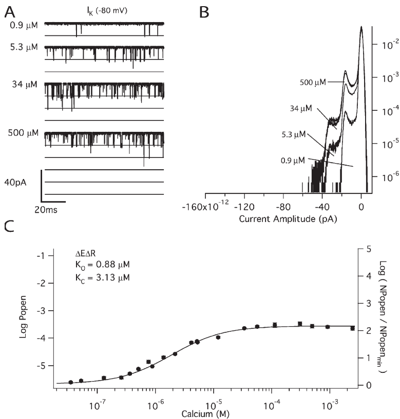
Figure 5. The \text{Ca}^{2+} binding affinities of the \text{Ca}^{2+} bowl site at -80 mV. (A) Inward \text{K}^+ currents recorded from mutant \Delta E\Delta R at -80 mV and filtered at 10 kHz from a macropatch exposed to the indicated [\text{Ca}^{2+}] demonstrate that Popen increases in a \text{Ca}^{2+} -dependent manner when voltage is constant. The corresponding all-point amplitude histograms are plotted in B on a semi-log scale and were constructed from 30-s recordings as in Fig. 2. The dose-response relation for the effect of [\text{Ca}^{2+}] on Popen (left axis) and \text{NPopen}/\text{NPopen}_{\text{min}} (right axis) at negative voltage ( -80 mV) is shown in C. Each point represents the average of between 6 and 11 patches at each [\text{Ca}^{2+}] tested. \log(\text{NPopen}/\text{NPopen}_{\text{min}}) spans the entire [\text{Ca}^{2+}] range and is fit (solid line) by Eq. 6 yielding values of K_O = 0.88 \mu\text{M} and K_C = 3.13 \mu\text{M} . Error bars represent SEM.
