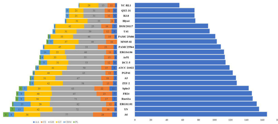
Fig. 4 Comparative CAZyme-encoding genes found in the genome of Arthrobacter species. On the left side is the CAZyme family and on the right side is the total CAZyme number: GT, glycosyltransferase; GH, glycoside hydrolase; CE, carbohydrate esterase; CBM, carbohydrate-binding modules; and AA, auxiliary activity. The CAZyme family is colored, as indicated below the figure. Arthrobacter sp.: PAMC25564, 24S4-2, YN, QXT-31, Rue61a, FB24, PAMC25486, ZXY-2, U41, DCT-5, PGP41, ERGS1:01, YC-RL1, Hyio4, KBS0702, UKPF54-2, MN05-02, Hyio8, and ATCC21022 Arthrobacter crystallopoietes : DSM 20117 Arthrobacter alpinus : R3.8, ERGS4:06, and A3 Pseudarthrobacter phenanthrenivorans : Sphe3 Pseudarthrobacter chlorophenolicus : A6 and Pseudarthrobacter sulfonivorans : Ar51
