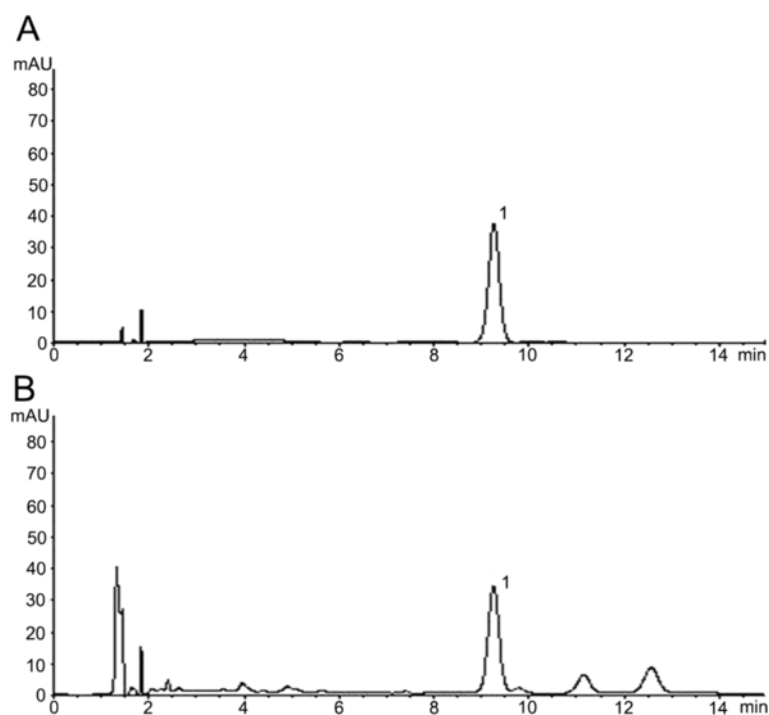
Figure 1 Chromatograms for \beta -ecdysone (A) and 80% ethanol extract of Achyranthes bidentata (B).
