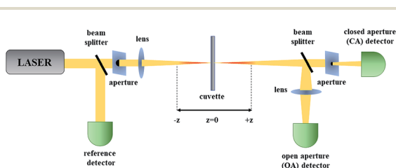
Fig. 4 The scheme of a Z-scan setup. OA – open aperture for measurement of nonlinear absorption; CA – closed aperture for measurement of nonlinear refractive index.
