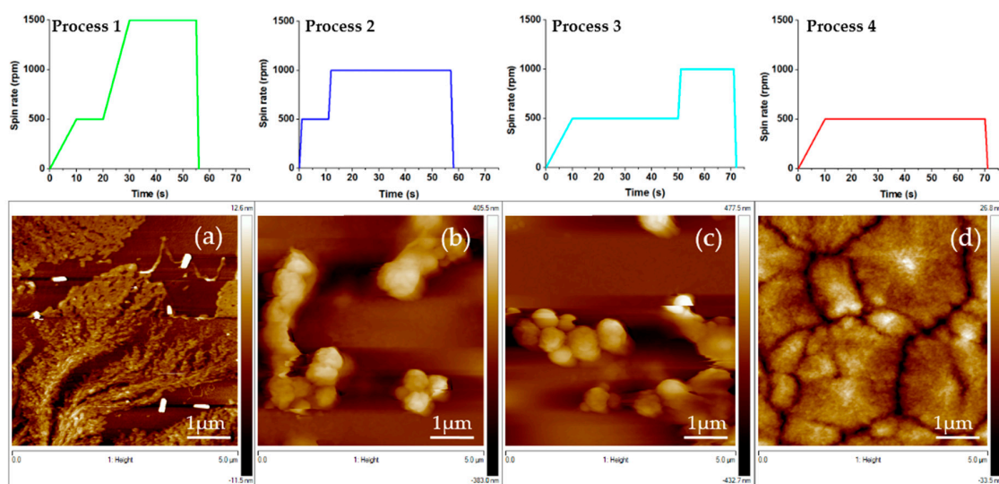
Figure 2. 5 \times 5 \mu\text{m} AFM micrographs showing the morphology of PVDF spin-coated thin films with the corresponding spin coating processes on the top. Bottom: thin film obtained (a) by process 1; (b) by process 2; (c) by process 3; (d) by process 4.
