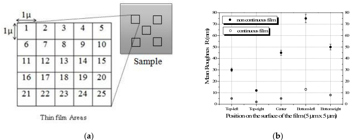
Figure A1. (a) Scheme of the 5 \times 5 \mu\text{m} AFM micrograph analysis. Each sample surface imaged by AFM standard microscope, has been divided in five zones (see the right top of the figure (a)) and each of these zones has been analyzed in order to obtain a roughness value for each 1 \times 1 \mu\text{m} square reported in the scheme. (b) The mean roughness value of each zone is here reported as function of the five different zones analyzed for two different kinds of samples (continuous and not continuous).
