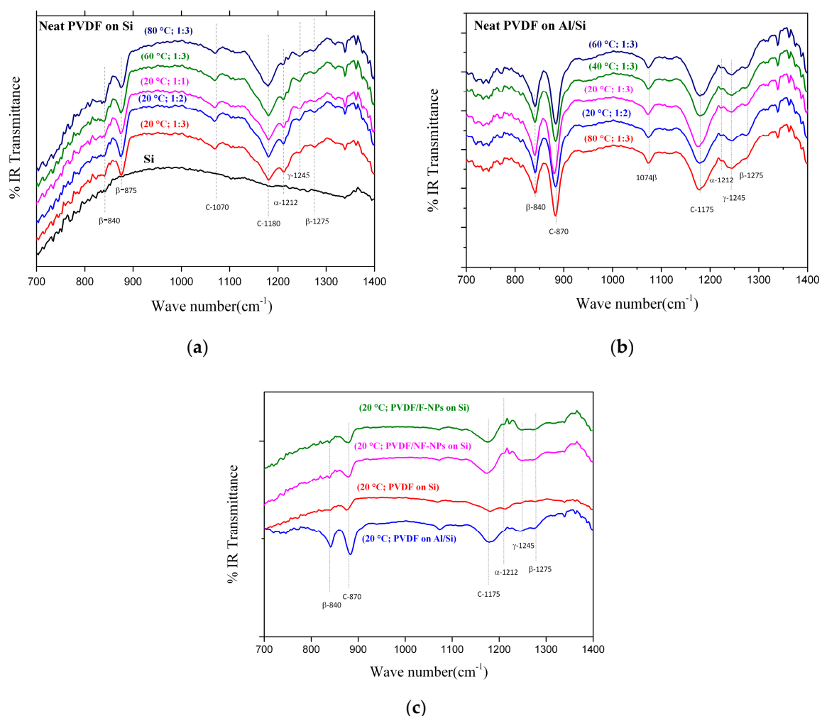
Figure 7. (a) IR transmittance of neat PVDF thin films on Si substrate with different elaboration parameters detailed in parenthesis (temperature; DMF/acetone ratio); (b) IR transmittance of neat PVDF thin films on Al/Si substrate with different elaboration parameters detailed in parenthesis (temperature; DMF/acetone ratio); (c) comparison between neat PVDF thin films on Si and Al/Si and composite thin films obtained by equal conditions of elaboration with functionalized (F-NPs) nanoparticles and non-functionalized ones (NF-NPs).
