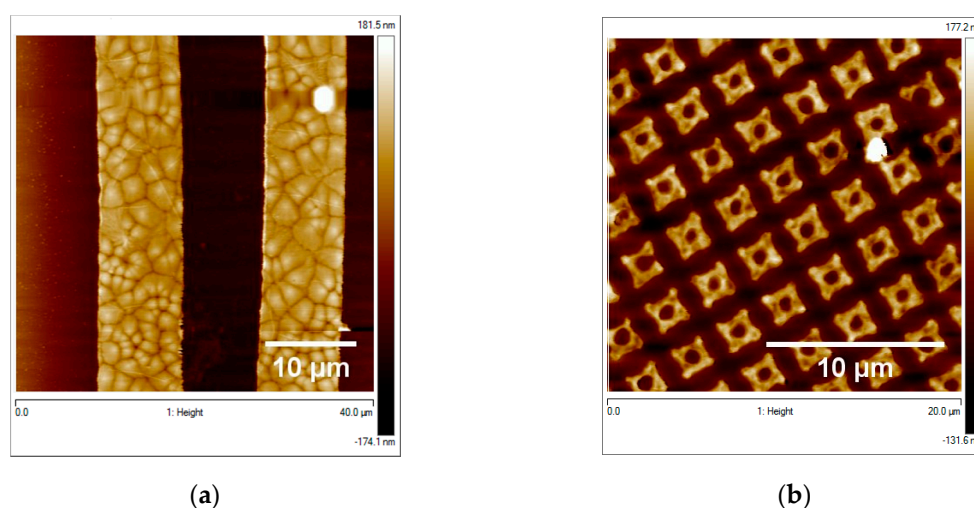
Figure 9. (a) 40 \times 40 \mu\text{m} AFM micrograph of the 10 \mu\text{m} micro lines of PVDF; (b) 20 \mu\text{m} AFM micrograph of the 2 \mu\text{m} diameter squared-rings.
