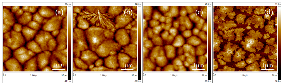
Figure 4. 5 \times 5 \mu\text{m} AFM micrographs showing the morphology of PVDF thin films spin-coated on silicon at different temperature: PVDF films obtained at (a) 20 °C; (b) 40 °C; (c) 60 °C and (d) 80 °C.
