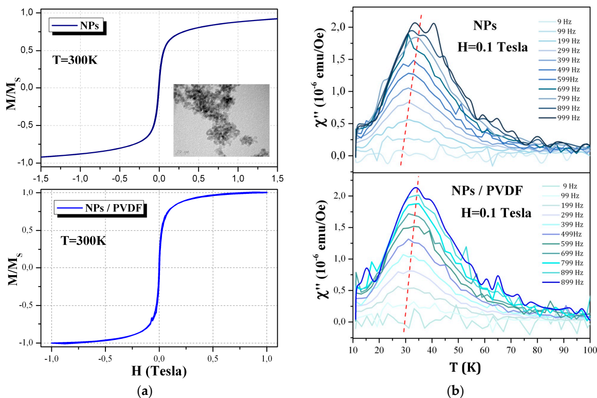
Figure 8. (a-top) hysteresis cycle at room temperature of Co-based nano-inclusions (inset: TEM image of the nanoparticles) and (a-bottom) composite film containing 1 wt % of functionalized nano-inclusions; (b-top) magnetic susceptibility as function of temperature for Co-based nano-inclusions and (b-bottom) composite film containing 1 wt % of functionalized nano-inclusions.
