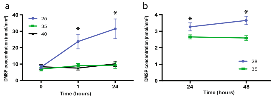
Fig. 2 Changes in DMSP concentration (mean \pm s.e.) in adult corals ( n = 5 ) and settled juveniles ( n = 6 ) of the coral A. millepora . Adults (a) were exposed to ambient/control (35 PSU, green) and two salinity stress conditions (25 and 40 PSU in blue and black respectively). DMSP concentrations increased significantly under hyposaline stress (25 PSU; *H-F Pr < 0.005) and through time compared to both the control and hypersaline stress conditions (40 PSU; *p adj < 0.05). No significant changes in DMSP levels were observed between the control and 40 PSU treatments. Juveniles (b) were exposed to ambient/control (35 PSU, green) or hyposaline (28 PSU, blue) conditions. In this case, DMSP levels differed significantly between treatments and controls ( F = 17.70 , * p < 0.0005 ), but did not differ significantly with time
