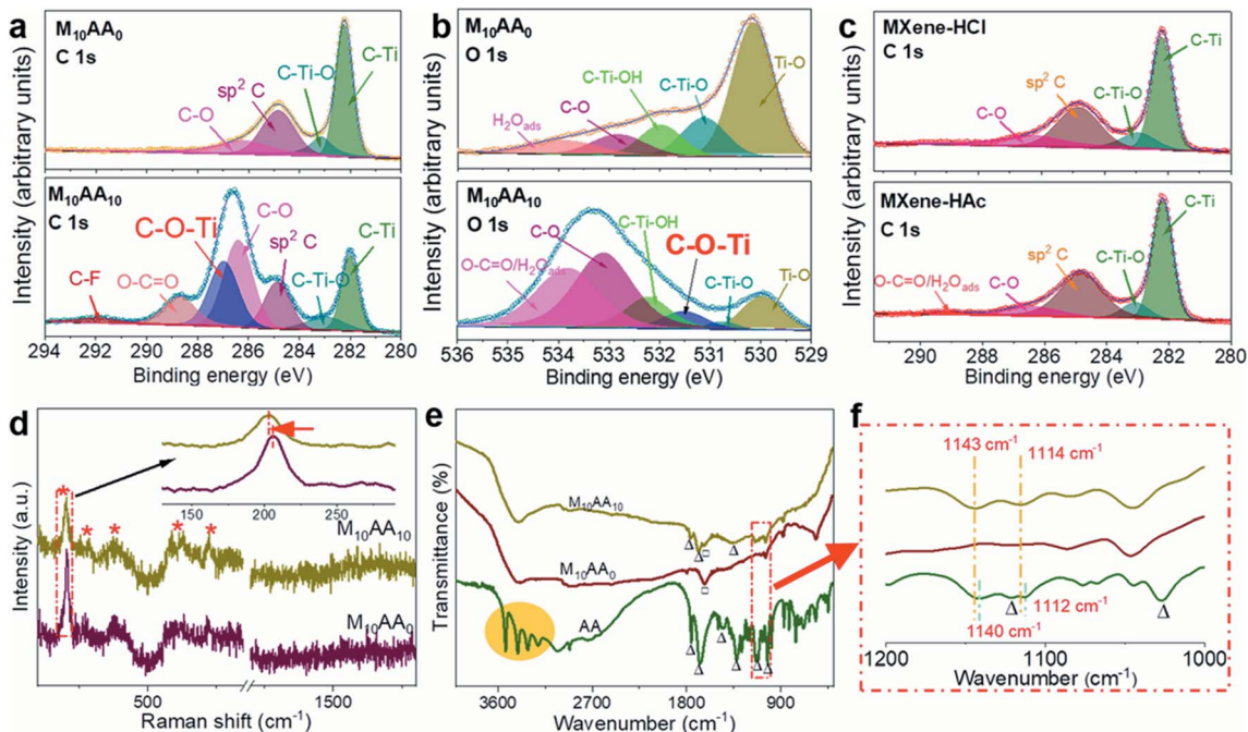
Fig. 4 (a) High-resolution C 1s spectra and (b) O 1s spectra of M 10 AA 0 and M 10 AA 10 ; (c) high-resolution C 1s spectra of MXene treated with HCl and with HAC; (d) Raman spectra of M 10 AA 0 and M 10 AA 10 ; (e) and (f) FTIR spectra of M 10 AA 0 , M 10 AA 10 and AA (where "Δ" stands for characteristic peaks for AA and "□" for Ti 3 C 2 T x MXene, details on the assignment of FTIR peaks are given in Fig. S6†).
