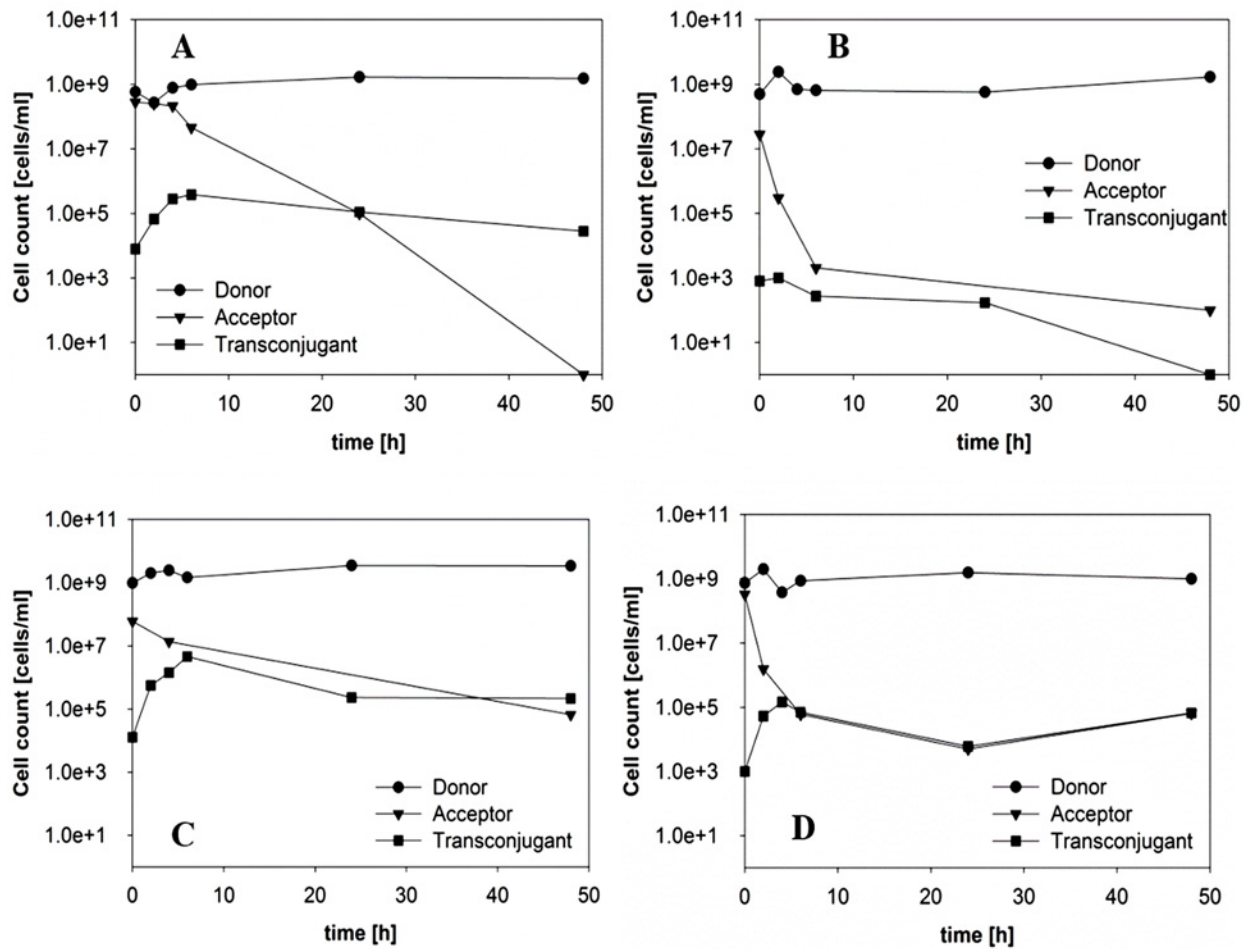
Fig 5. Transfer of pESBL-283 from ESBL242 (donor, amp R ) to E. coli MG1655 (acceptor, chlor R ). After donor and acceptor cells reached steady states in separate chemostats, cultures were mixed in a ratio of 1:1 in an empty reactor vessel and immediately supplied with fresh medium at the same dilution rate. Experimental conditions in each of the panels: (A) 0 μg/ml at D = 0.2 h -1 , (B) 512 μg/ml ampicillin at D = 0.2 h -1 , (C) 0 μg/ml at D = 0.4 h -1 and (D) 512 μg/ml ampicillin at D = 0.4 h -1 .
