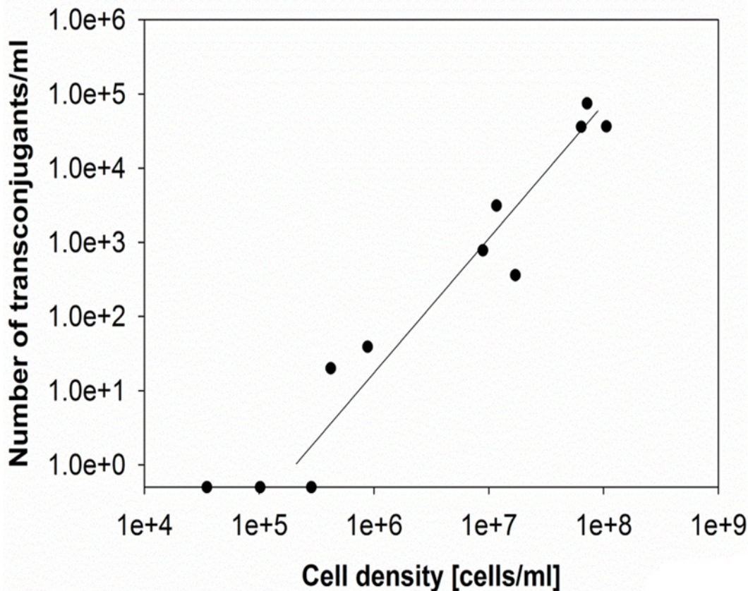
Fig 1. Number of evolved transconjugants/ml after co-culturing ESBL242 (donor, amp R ) and E. coli MG1655 (acceptor, chlor R ). Cells were mixed in a ratio of 1:1 at different total cell densities and incubated for 1 hour in batch culture.
