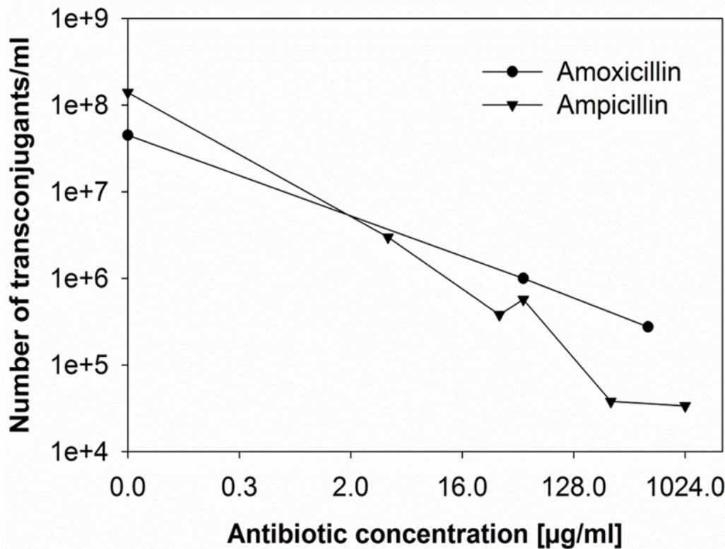
Fig 3. Number of evolved transconjugants/ml after co-culturing ESBL242 (donor, amp R ) and E. coli MG1655 (acceptor, chlor R ) for 24 hours in batch culture. Cells were mixed in a ratio of 1:1 with varying antibiotic concentrations.
