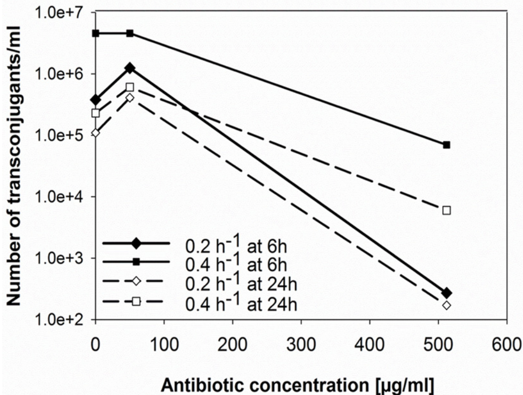
Fig 6. Number of transconjugants during continuous cultivation of ESBL242 (donor) and E. coli MG1655 (acceptor) cells at t = 6h or 24h. E. coli MG1655 and ESBL242 cells were cultivated separately and continuously at a dilution rate of D = 0.2 or 0.4 \text{ h}^{-1} and subsequently mixed with a ratio of 1:1 ( t = 0\text{h} ).
