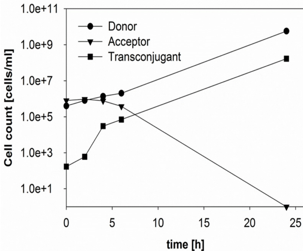
Fig 4. Transfer of pESBL-283 from ESBL242 (donor, amp R ) to E. coli MG1655 (acceptor, chlor R ) in a ratio of 1:1 with 8 µg/ml ampicillin and 4 µg/ml clavulanic acid.
