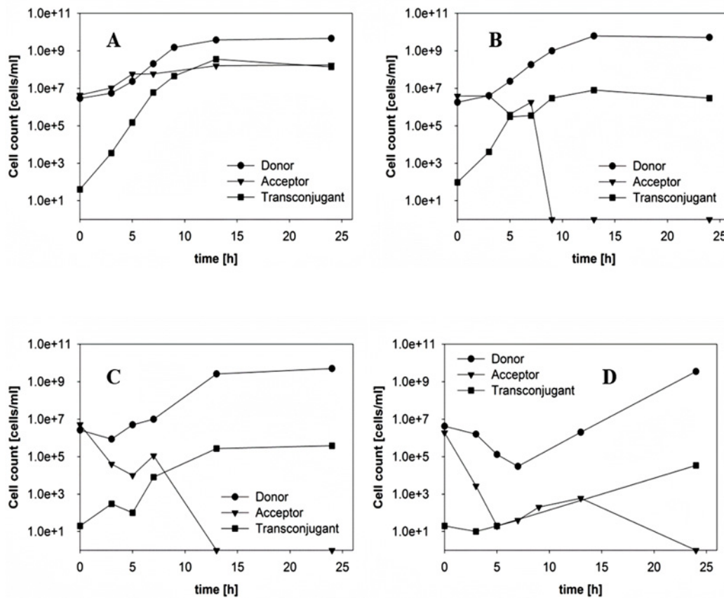
Fig 2. Transfer of pESBL-283 from ESBL242 (donor, amp R ) to E. coli MG1655 (acceptor, chlor R ) as a function of time during co-culture in a ratio of 1:1 with (A) 0 µg/ml, (B) 4 µg/ml, (C) 32 µg/ml and (D) 1024 µg/ml ampicillin in batch culture.
