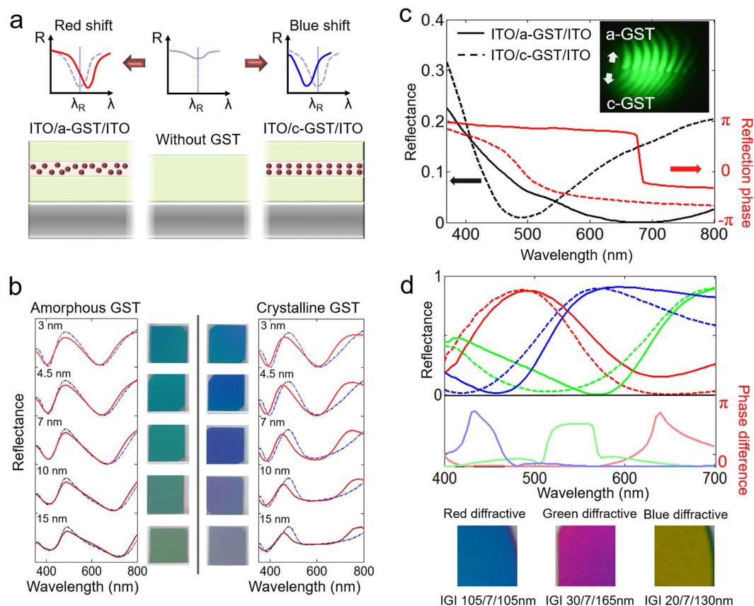
Figure 3. (a) Schematic diagram for illustrating the major variation of the optical spectrum when amorphous (or crystalline) thin GST film is inserted into ITO on a metal substrate. (b) Simulation (blue dash-dotted) and experimental (red solid) results of the reflection spectra to observe the effects of the GST thickness. (c) Reflectance and reflection phase of the IGI composite layer designed for broadband visible light diffraction (IGI 30/7/30 nm). The upper-right inset shows the abrupt phase difference of reflected light as measured by a Michelson interferometer experiment. (d) The upper-side plots show the experimental results of the reflection spectra for amorphous (solid lines) and crystalline (dashed lines) GST inserted panels designed for red, green, and blue color-selective diffraction. The lower-side plots show the numerical results of the reflection phase difference |\angle r_{am} - \angle r_{cry}| between the amorphous and crystalline GST insertion cases. The bottom images show the color of reflection panels and their IGI thickness conditions.
