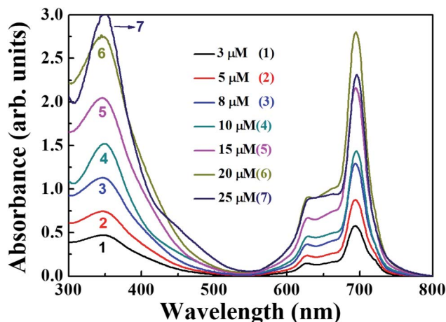
Fig. 3 Absorption spectral changes of PBIPC in THF at different concentrations of (1) 3 \mu\text{M} , (2) 5 \mu\text{M} , (3) 8 \mu\text{M} , (4) 10 \mu\text{M} , (5) 15 \mu\text{M} , (6) 20 \mu\text{M} and (7) 25 \mu\text{M} .
