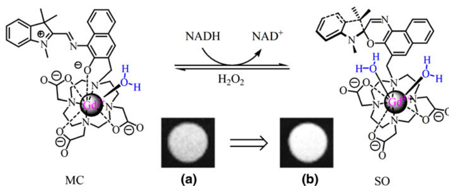
FIGURE 9. The structural and hydration number ( q ) changes in the first coordination sphere of Gd(III) of spirooxazine-Gd-DO3A triggered by NADH and hydrogen peroxide. T_1 -weighted MRI images of (a) spirooxazine-Gd-DO3A and (b) the mixture of spirooxazine-Gd-DO3A and NADH (Gd:NADH = 1:1), in P388D1 murine macrophages. Images modified from Scheme 2 and Fig. 5 in Tu et al. 80 .
