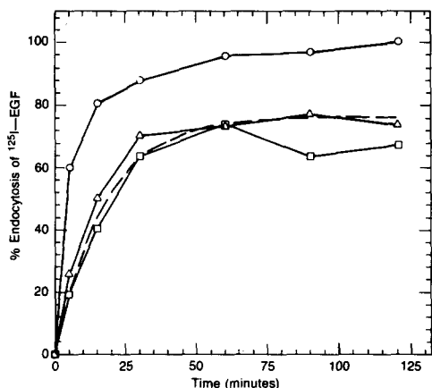
Figure 2. Relative internalization of [ ^{125} I]EGF was determined by taking the ratio of cpm resistant to the acetic acid wash to total cpm determined by binding [ ^{125} I]EGF at 4°C (see Materials and Methods) ( \square ) represents values obtained for HER82; ( \Delta ) for HER22; and ( \circ ) for HER84 cell lines, respectively. The total number of internalized receptors is simulated by assuming partial recovery of recycled coated-pits. Taking e_0 = 2.9 \times 10^5 sites initially occupied by receptors and internalized, and e_1 = qe_0 sites recycled and restored after five minutes, we get for the total number of internalized receptors after T minutes (or T/5 cycles):
