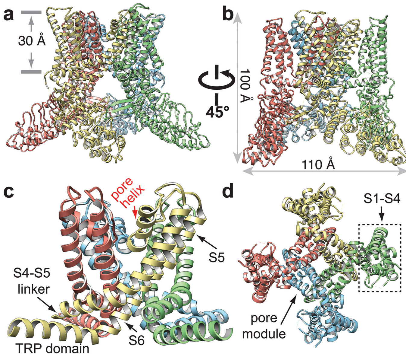
Figure 2. TRPV1 and VGICs share similar 4-fold symmetric architecture
