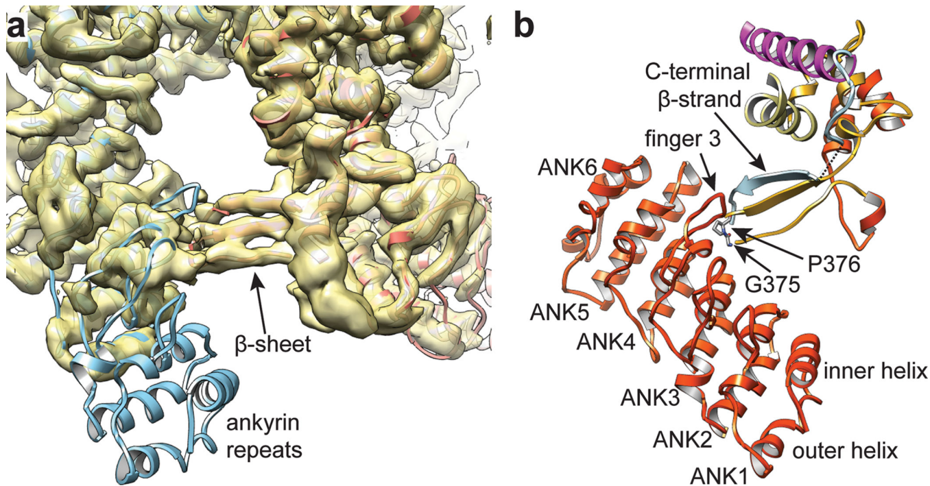
Figure 6. Cytosolic interactions mediated by ankyrin repeat domains
