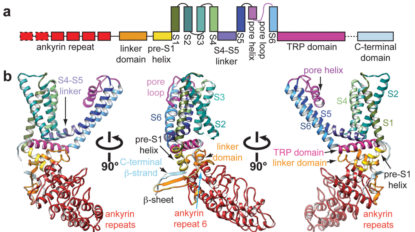
Figure 3. Structural details of a single TRPV1 subunit
