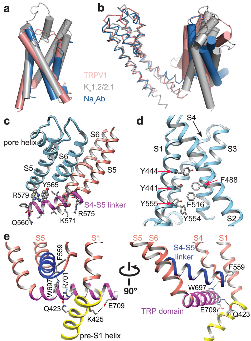
Figure 4. Unique structural features of TRPV1
