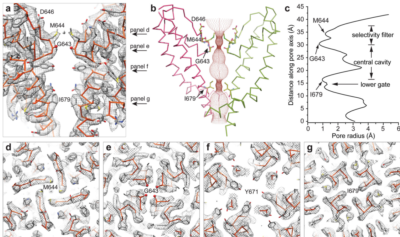
Figure 5. The ion permeation pathway of TRPV1
