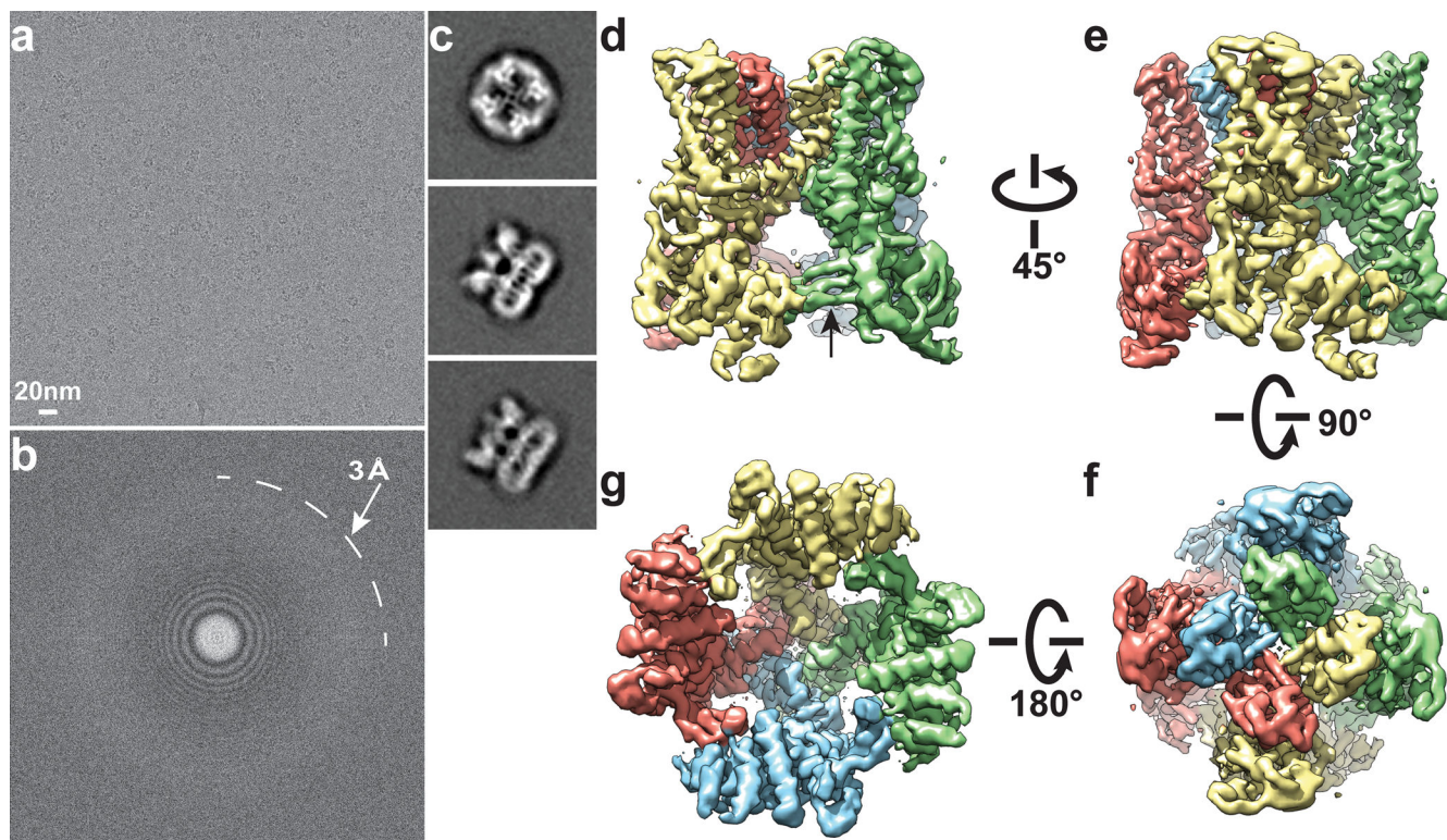
Figure 1. 3D reconstruction of TRPV1 determined by single-particle cryo-EM
