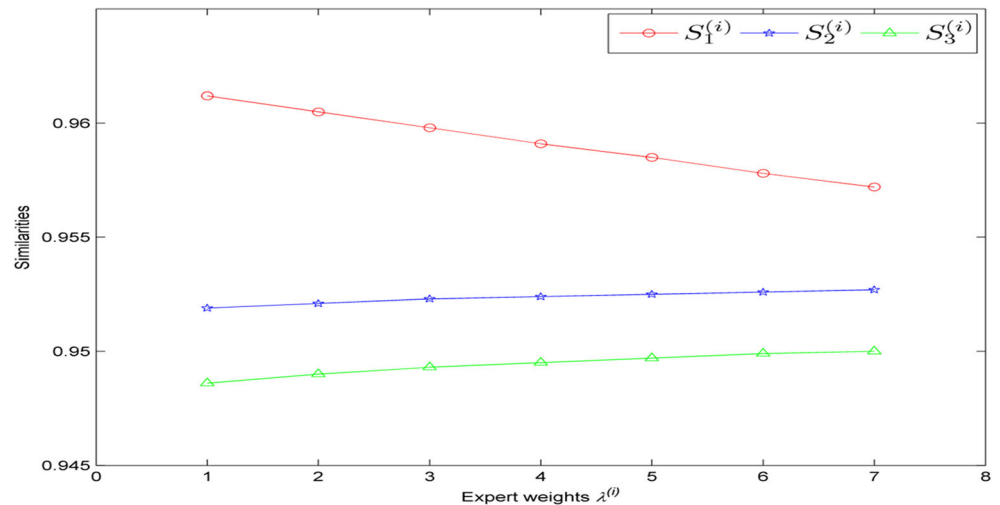
Fig. 4 Influence of adjusting expert weights to PrHPFM similarities
