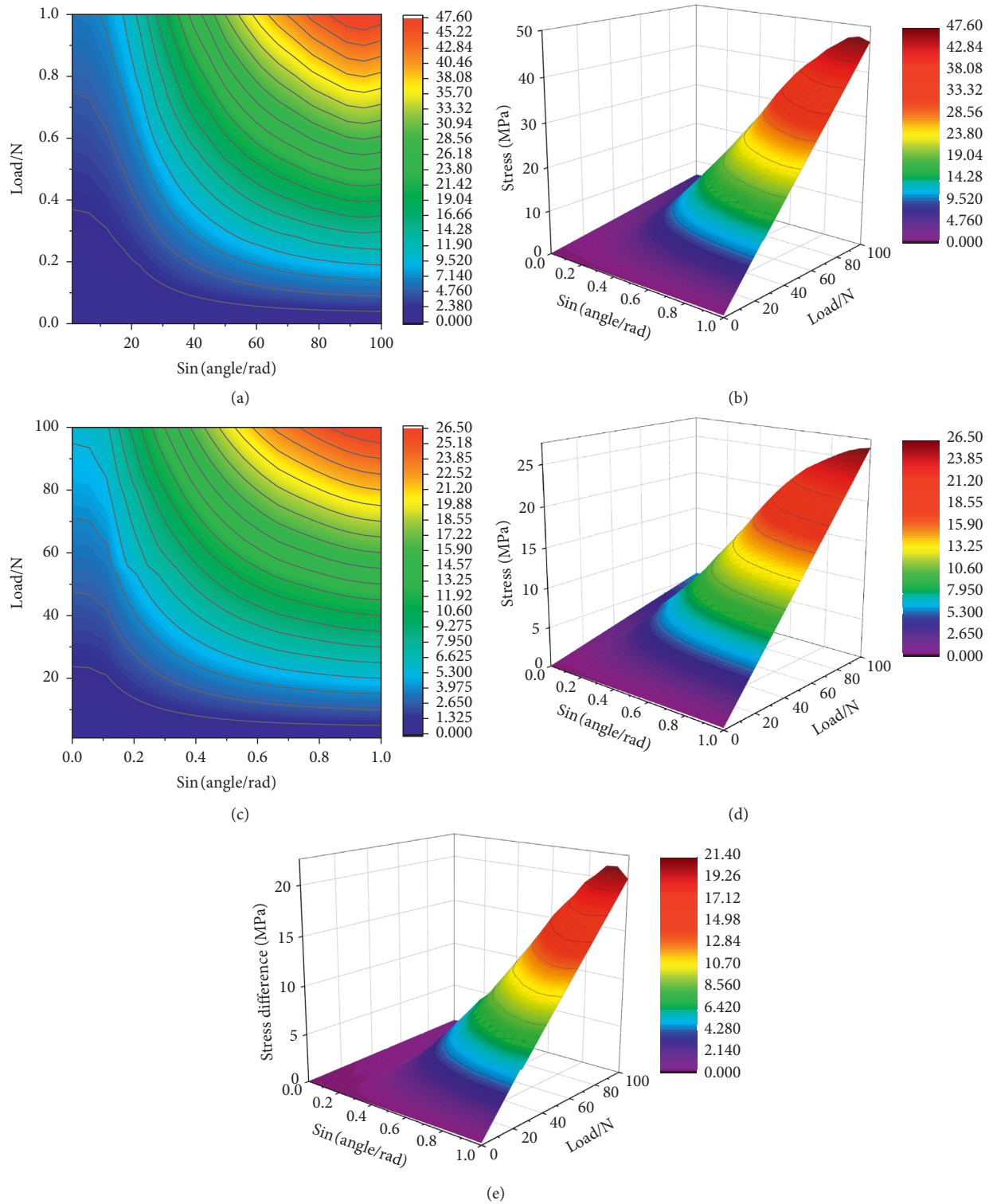
FIGURE 3: Quantitative relation between the loading force and stress on the cortical bone and abutment. (a) Von Mises contour map of the ROI of the abutment under different magnitudes and angles of loading forces. (b) 3D surface of the abutment under different magnitudes and angles of loading forces. (c) Von Mises contour map of the ROI of the alveolar bone under different magnitudes and angles of the loading forces. (d) 3D surface of the alveolar bone under different magnitudes and angles of loading forces. (e) 3D surface of the stress differences of the abutment and alveolar bone under different magnitudes and angles of loading forces.
