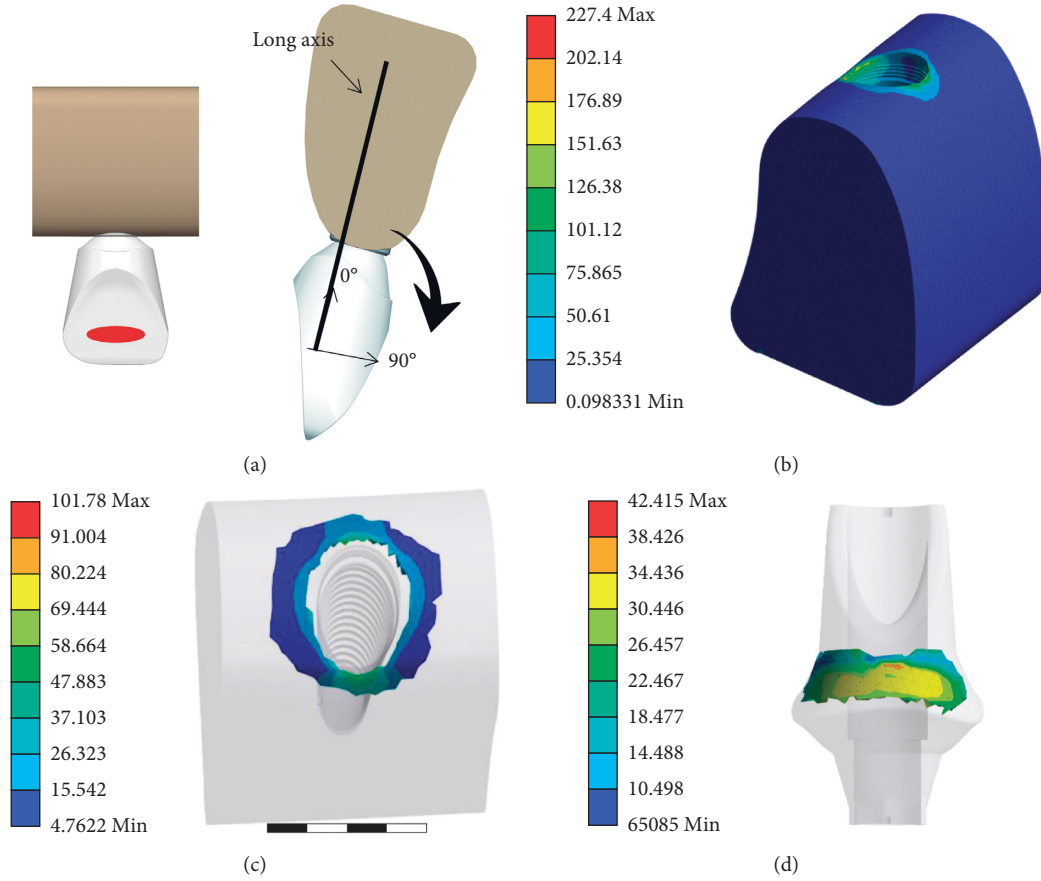
FIGURE 2: The condition of loading force and selection of the region of interest (ROI) of the alveolar bone and abutment. (a) Loading force position and loading force angle. (b) The region of stress concentration on the alveolar bone. (c) The ROI of the alveolar bone. (d) The ROI of the abutment.
