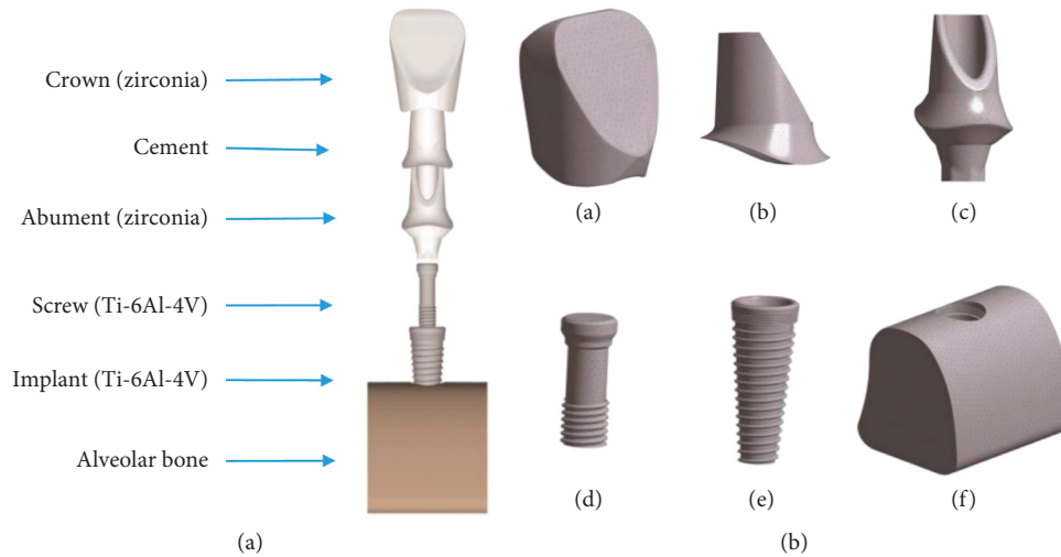
FIGURE 1: (a) 3D model of the implant system. (b) Finite element models of crown (a), cement (b), abutment (c), screw (d), implant (e), and alveolar bone (f).
