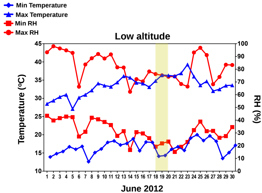
Supplementary Figure S1. Daily climate record (max/min temperature and relative humidity) in high- and low-altitude regions. Colored boxes indicate the harvest period in each region.
