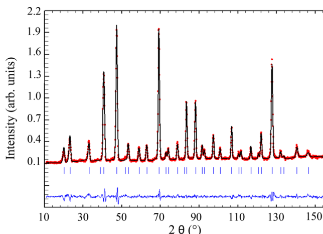
Figure 2. Comparison between the calculated ( Y_{\text{calc}} , in black) and observed ( Y_{\text{obs}} , in red) neutron diffraction patterns of \text{Ba}_2\text{NaMoO}_{5.5} . Y_{\text{obs}} - Y_{\text{calc}} (in blue) is the difference between the observed and calculated intensities. The angular positions of Bragg reflections are shown in blue. The measurement has been performed at \lambda = 1.667 \text{ \AA} .
