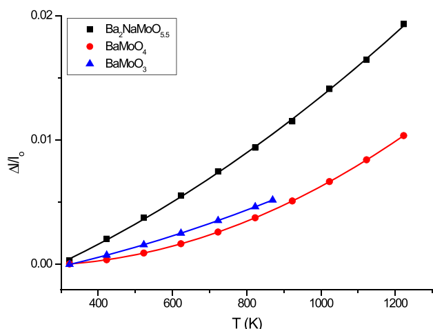
Figure 6. Relative thermal expansion of Ba 2 NaMoO 5.5 , compared to BaMoO 4 31 and BaMoO 3 . 32
