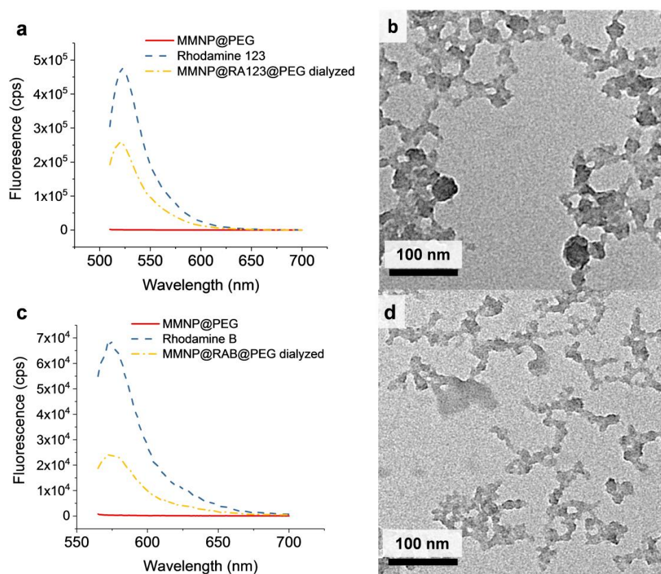
Figure 6. Fluorescence emission spectra and TEM images of in situ labeled MMNP@RA123 and MMNP@RAB. (a) Fluorescent emission spectra ( \lambda_{ex} = 500 nm) of MMNP@RA123@PEG after seven day dialysis in 1\times phosphate-buffered saline (PBS), rhodamine 123, and MMNP@PEG. (b) TEM image of MMNP@RAB. (c) Fluorescent emission spectra ( \lambda_{ex} = 555 nm) of MMNP@RAB@PEG after seven day dialysis in 1\times PBS, rhodamine B, and MMNP@PEG. (d) TEM image of MMNP@RA123.
