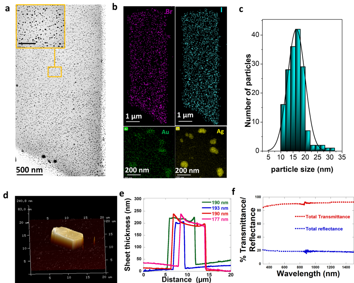
Fig. 3 Structural characterization of the composite. (a) TEM image of a CTAB-I sheet embedded with particles; inset shows the particles inside the sheet (scale bar 100 nm). (b) HAADF-STEM image of the particle-embedded CTAB-I sheet with the elemental mapping distribution of bromine, iodine (sheet), gold, and silver (embedded particles). (c) Histogram plot of the size distribution of particles that are embedded inside the sheet. (d) 3D AFM image of the CTAB-I sheet embedded with particles. (e) Thickness profile analysis of the sheet. (f) Optical reflectivity and transmissivity of CTAB-I sheets with particles.
