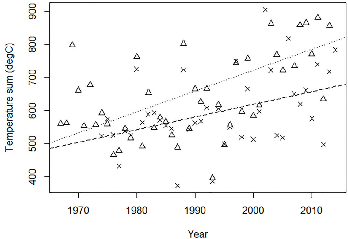
Fig 4. Temperature sums (°C) for the continental (1974–2014; crosses) and oceanic (1967–2014; triangles) sites. Points show temperature sums measured each year at both sites. Regression lines are plotted from linear models of the continental (dashed line: r^2 = 0.149 , P = 0.007 , n = 41 ) and oceanic (dotted line: r^2 = 0.340 , P < 0.001 , n = 48 ) site data.
