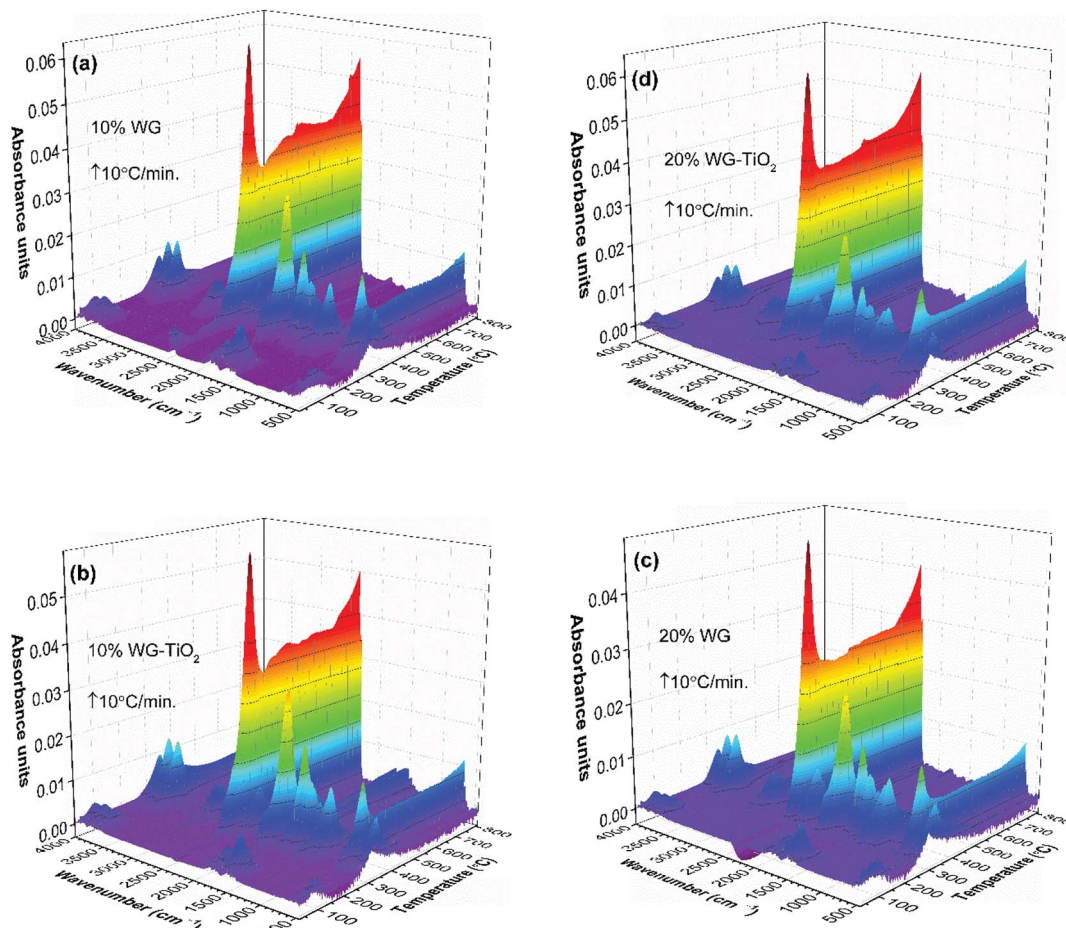
Fig. 5 TG-FTIR absorbance spectra 3D stack plots of the pyrolysis components of Scots pine sapwood modified with (a) 10% Na 2 SiO 3 , (b) 10% Na 2 SiO 3 -nTiO 2 , (c) 20% Na 2 SiO 3 , and (d) 20% Na 2 SiO 3 -nTiO 2 , as a function of temperature.
