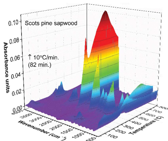
Fig. 4 TG-FTIR absorbance spectra 3D stack plot of unmodified Scots pine sapwood pyrolysis components as a function of temperature.
