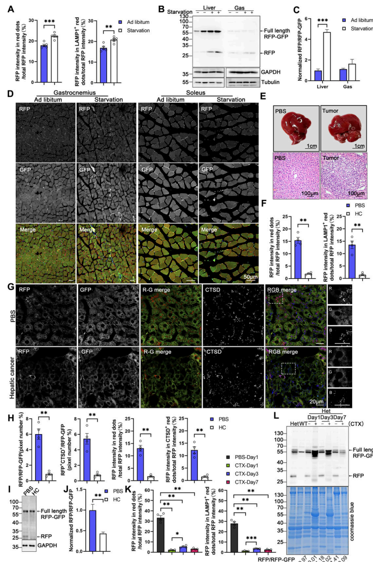
Figure S4. Assessment of ER-phagy in physio-pathological perturbations (related to Fig. 8). (A) Quantitative analysis indicated increased RFP + and RFP + LAMP1 + signals at liver during starvation. The fluorescence intensity of RFP-only, RFP + LAMP1 + and total area were calculated respectively by ImageJ and the fluorescence ratio of RFP-only (or RFP + LAMP1 + ): the total RFP was quantified. Values were stated as mean ± SEM ( n = 5 per condition). Statistical differences were analyzed using Student's t test. ** P < 0.01, *** P < 0.001. (B and C) Analysis of ER-phagy levels in the liver and skeletal muscle of transgenic mice during starvation by immunoblotting. Tissue homogenates from both regularly fed and starved mice were examined through immunoblotting. Full-length RFP-GFP and RFP fragments were detected with an anti-RFP antibody and the band intensity of RFP fragments relative to full-length RFP-GFP indicates the presence of ER-phagy products, signifying ER-phagy activity. GAPDH and Tubulin served as internal controls. Adult male wild-type and ER-TRG (+/-) mice were used in experiments. Values were stated as mean ± SEM ( n = 4 per condition). Statistical differences were analyzed using two-way ANOVA. *** P < 0.001. (D) Confocal imaging of RFP and GFP signals in the skeletal muscles (gastrocnemius, soleus) of ER-TRG (+/-) mice under normal feeding and starvation. Scale bar: 50 µm. (E) Hematoxylin and Eosin (HE) staining of liver sections from PBS-treated and hepatic cancer model mice in ER-TRG (+/-) mice. Control mice received PBS injections, while model mice were injected with plasmids expressing C-Myc, N-Ras, and SB11 for 4 wk. Scale bars: 1 cm (top), 100 µm (bottom). (F) Quantitative analysis indicated reduced RFP + and RFP + LAMP1 + signals at tumor sites compared with control liver or adjacent tissue. The fluorescence ratio of RFP-only (or RFP + LAMP1 + ): the total RFP was quantified. Values were stated as mean ± SEM ( n = 4 per condition). Statistical differences were analyzed using Student's t test. ** P < 0.01. (G and H) ER-phagy levels and quantitative analysis in the liver of ER-TRG (+/-) mice with hepatic cancer. Confocal imaging reveals diminished ER-phagy at tumor sites relative to control liver or adjacent tissues, as indicated by CTSD co-staining. The pixel number, fluorescence intensity of RFP-only, RFP+CTSD+ and total area were calculated by ImageJ. The ratio of RFP-only (or RFP+CTSD+): the total area (RFP+GFP) and the fluorescence ratio of RFP-only (or RFP+CTSD+): the total RFP were quantified. Values were stated as mean ± SEM ( n = 4 per condition). Statistical differences were assessed using Student's t test. ** P < 0.01. Scale bar: 20 µm. (I and J) Analysis of ER-phagy levels in the liver of ER-TRG (+/-) mice with hepatic cancer by immunoblotting. Values were stated as mean ± SEM ( n = 4 per condition). Statistical differences were analyzed using Student's t test. ** P < 0.01. (K) Quantitative analysis indicated altered RFP + and RFP + CTSD + signals in muscle cells at injury area compared to PBS-treated tissue. The fluorescence ratio of RFP-only (or RFP + LAMP1 + ): the total RFP was quantified. Values were stated as mean ± SEM ( n = 4 per condition). Statistical differences were analyzed using one-way ANOVA and Kruskal–Wallis test. * P < 0.05, ** P < 0.01, *** P < 0.001. (L) Analysis of ER-phagy levels in the skeletal muscle of ER-TRG (+/-) mice with CTX injury by immunoblotting. The band intensity of RFP fragments relative to full-length RFP-GFP indicates the presence of ER-phagy products, signifying ER-phagy activity. Coomassie blue staining confirmed protein loading. Adult male wild-type and ER-TRG (+/-) mice were used in experiments. Source data are available for this figure: SourceData FS4.
