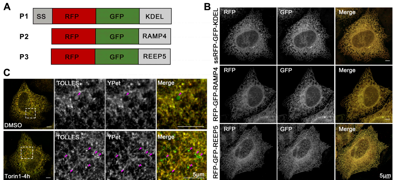
Figure S1. Expression of different ER-phagy reporters in cell line (related to Figs. 1, 2, and 3). (A) Schematic depiction of several ER-phagy reporter candidates. Each reporter incorporates the tandem fluorescent protein RFP-GFP. P1 features the RFP-GFP tandem along with the ER-lumen targeting sequence SS-KDEL. P2 consists of RFP-GFP paired with the sheet ER-membrane protein RAMP4. P3 includes RFP-GFP combined with the tubular ER-membrane protein REEP5. (B) Confocal microscopy images of HeLa cells expressing various ER-phagy reporters. HeLa cells transiently expressing each of the three reporters (P1-P3) were examined to characterize ER morphology. Scale bar: 5 µm. (C) Representative confocal microscopy images of ER-phagy in HeLa cells expressing ssYPet-TOLLES-KDEL following ER-stress inducer treatment. Cells transiently expressing ssYPet-TOLLES-KDEL were treated with 100 nM Torin1 for 4 h to induce ER-phagy. For TOLLES imaging, excitation was at 445 nm with fluorescence detection at 460–500 nm. For YPet, excitation was at 514 nm and fluorescence was detected at 530–580 nm. The pink arrowheads indicate the ER-phagy sites. Scale bar: 5 µm.
