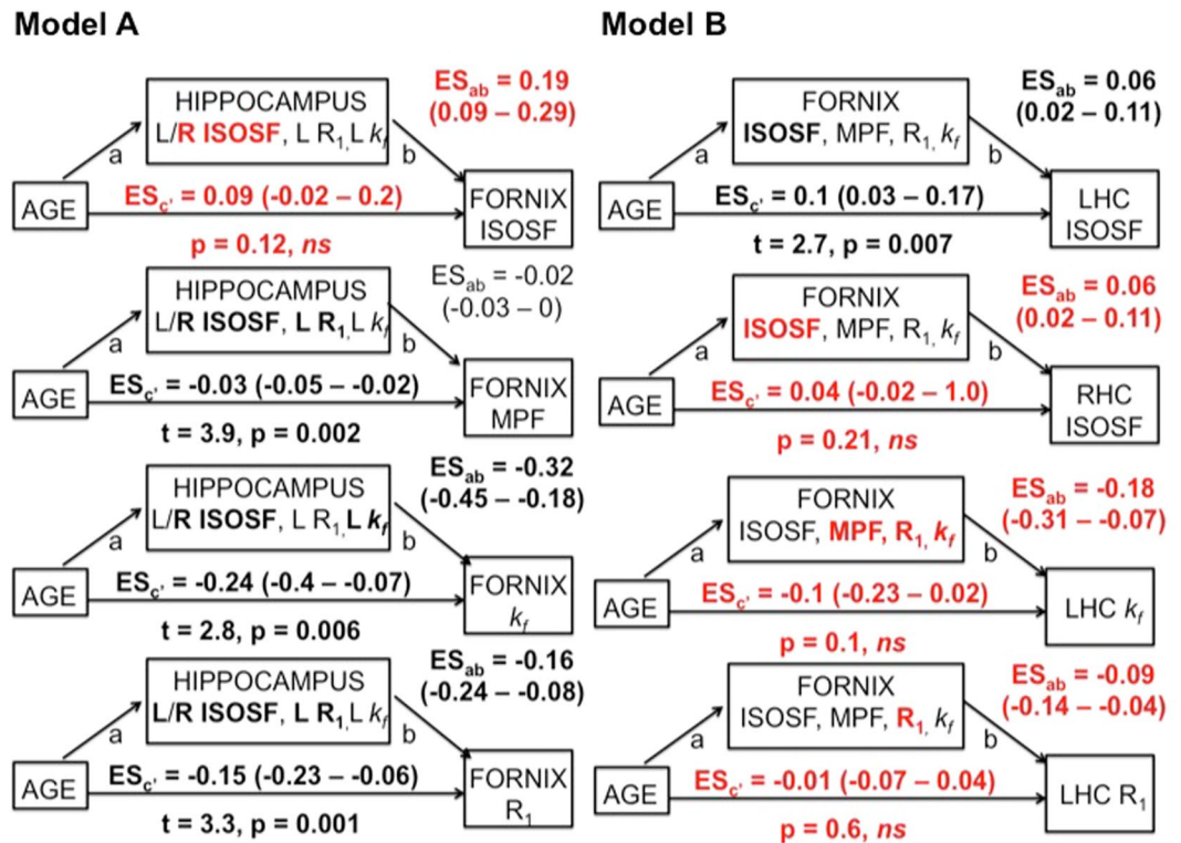
Figure 4. Summarises the results of the mediation analyses for Models A and B. 95% confidence intervals of the effect sizes ( ES \times 10^{-1} ) were based on bootstrapping with 5000 replacements. Fornix mediators in Model B had significant indirect effects and fully mediated the direct age effects on right hippocampal (RHC) isotropic signal fraction (ISOSF), left hippocampal (LHC) R 1 and k f (highlighted in red). In contrast, hippocampal mediators, although showing significant indirect effects (highlighted in bold), did not fully mediate the direct age effects on fornix MPF, R 1 and k f . Right (R) hippocampal ISOSF fully mediated fornix ISOSF and vice versa but fornix mediators did not remove the age effect on left hippocampal ISOSF. Mediator variables that contributed significantly to the regression analyses after 5% FDR correction are highlighted in bold.
