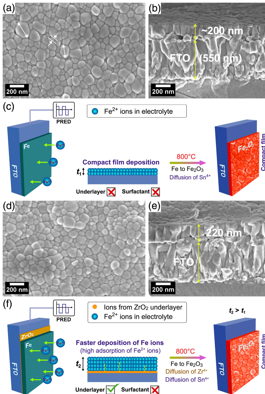
Figure 2. Surface and cross-sectional FESEM images of \text{Fe}_2\text{O}_3 photoanodes prepared with (a,b) F and (d,e) FZ conditions. Figure (c,f) shows the schematic of film formation on FTO for F and FZ conditions, respectively.
