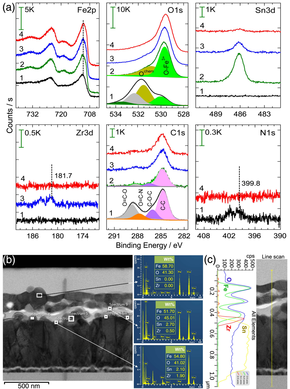
Figure 4. (a) High resolution XPS spectra of Fe2p, O1s, Sn3d, and Zr3d for as-grown (Curve 1: FZC) and annealed (Curve 2: F, 3: FZ, 4: FZC) films, (b) Cross-sectional TEM micrograph of annealed FZC sample with point EDS spectra revealing the % compositions of Fe, O, Sn and Zr elements, and (c) TEM-EDS line profile revealing the gradual diffusion doping of Sn and Zr ions.
