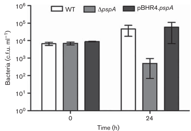
Fig. 3. Intracellular survival of stationary phase B. pseudomallei in J774A.1 macrophages. Macrophage cells were infected with 1 \times 10^7 c.f.u. ml -1 bacteria for 30 min, followed by incubation with 1 mg kanamycin ml -1 for 1 h to kill any extracellular bacteria. The cells were maintained in the presence of 250 \mu g kanamycin ml -1 and periodically lysed in order to enumerate the number of intracellular bacteria. Values are the mean \pm SEM from at least three independent experiments; * P <0.05.
