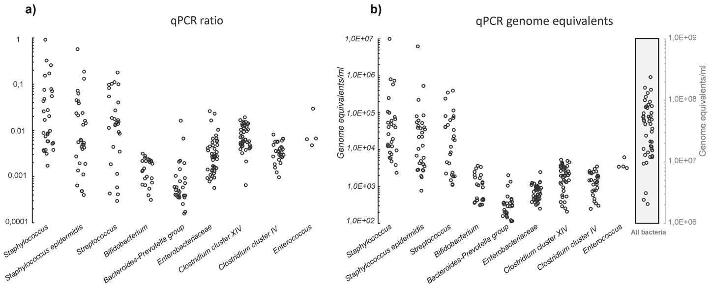
Fig 3. (a) Normalized distribution of detected bacterial groups across the sample set (one dot represents % of the detected group's specific DNA in relation to all bacterial DNA in the sample). (a, b). (b) Distribution of genome equivalents ml -1 colostrum for detected bacterial groups across the investigated maternal population.
