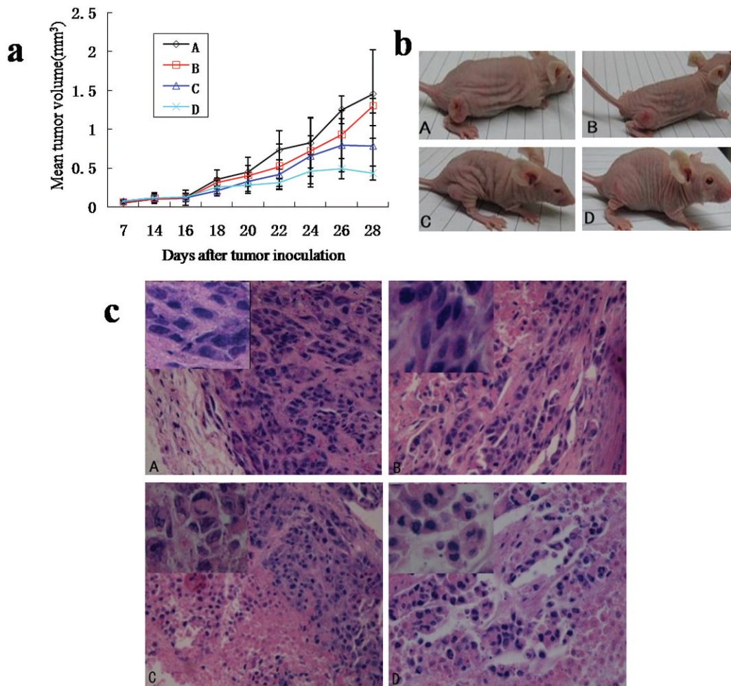
Figure 4 - Effect of curcumin on MDR in a HCT-8/VCR nude mice xenograft tumor model. Five-week-old female BALB/C nude mice were injected subcutaneously with HCT-8/VCR cells. Curcumin (50 mg/kg) and VCR (2 mg/kg) were administered twice daily through peritumoral injections for 14 days. After two weeks, the mice were sacrificed, and the tumors were harvested. A: control group; B: VCR group; C: curcumin group; D: curcumin+VCR group. (a) Effect of curcumin on the growth of HCT-8/VCR cells xenografted in nude mice, showing that curcumin inhibited tumor growth. (b) Representative tumor formation 14 days after intervention. (c) Hematoxylin-eosin staining of the tumors. (HE staining, ×200) A: control group; B: VCR group; C: curcumin group; D: curcumin+VCR group. The insets show magnified images representing typical changes of the tumor tissue.
