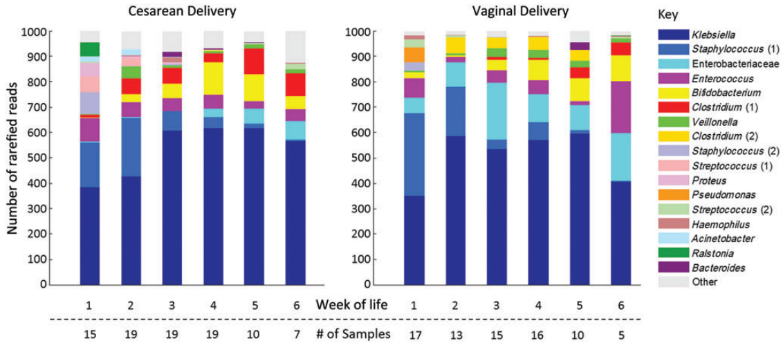
Figure 2. Bacterial community structure in control infants by postnatal week and mode of delivery. Data were generated using 1 sample per week from control infants using mean number of reads. When the same descriptive label (genus, family) is attached to >1 operational taxonomic unit (OTU; defined by 97% sequence similarity), these are numbered sequentially; no OTUs are combined.
