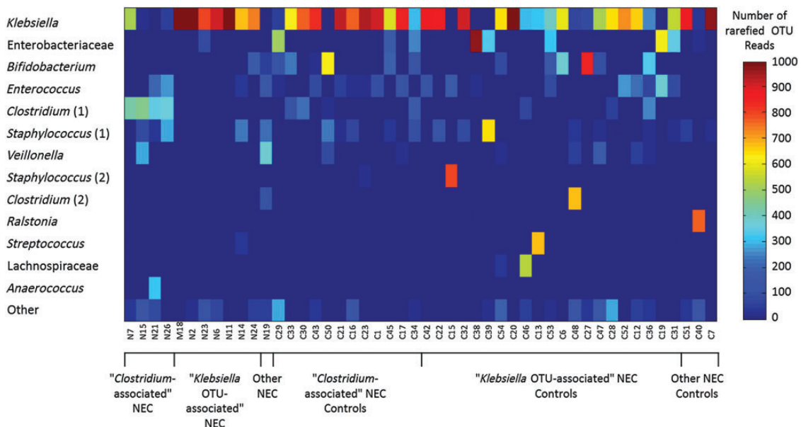
Figure 3. Bacterial communities in necrotizing enterocolitis (NEC) infant samples collected closest to the day of diagnosis of NEC ( D_0 ), and their matched controls. Samples are categorized along the x-axis. Color intensity indicates the number of rarefied reads from each operational taxonomic unit (OTU) that is found in a sample, as shown by the colored bar. Mean bacterial community diversity was not found to differ significantly between NEC and control infant samples.
