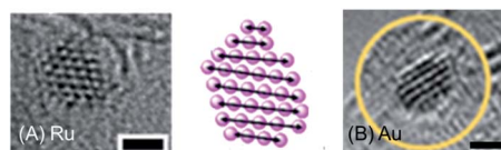
Fig. 4 Ruthenium and gold nanocrystals fabricated on a graphitic support by electron bombardment of \text{Ru(III)} and \text{Au(III)} complexes encapsulated in polymer micelles deposited on a lacey carbon EM grid in an aberration-corrected high-resolution transmission electron microscope. Interatomic distances: Ru–Ru 2.48 Å, Au–Au 2.73 Å. Scale bars 1 nm. Adapted from ref. 20 with permission from the Royal Society of Chemistry, copyright 2016. 20
