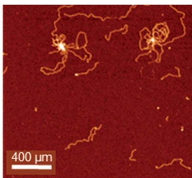
Fig. 8 pBR322 DNA plasmid deposited onto freshly cleaved mica treated with \text{Mg}^{2+} to ensure adsorption of the negatively-charged DNA. DNA condensation has been induced by the tetranuclear complex [\text{Os}_4(\eta^6\text{-}p\text{-cymene})_4(\mu^2\text{-OH})_4(\text{pyrazine})_2]^{4+} . Larger loops of DNA can also be seen. Adapted from ref. 37 with permission from Wiley-VCH, copyright 2016. 37
