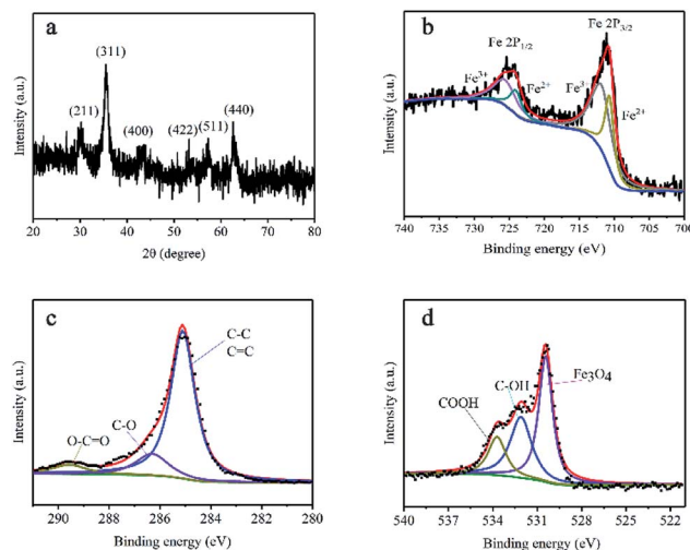
Fig. 3 (a) XRD pattern of SA/Fe 3 O 4 sample. (b–d) Fe 2p, C 1s and O 1s XPS core-level spectra of SA/Fe 3 O 4 sample.
