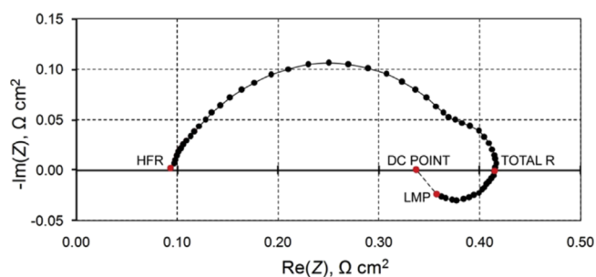
Figure 12. Impedance plot of a \text{H}_2/\text{air} PEM fuel cell (50 \text{cm}^2 , 65 °C, 0.5 bar(g), 15 A, \text{H}_2/\text{air} stoichiometry 2/4, 100% RH), high-frequency resistance, total R, DC point, and the last measured point. Reprinted from Pivac, I.; Šimić, B.; Barbir, F. Experimental diagnostics and modeling of inductive phenomena at low frequencies in impedance spectra of proton exchange membrane fuel cells. J. Power Sources 2017 , 365 , 240–248, with permission from Elsevier. Copyright (2017) Elsevier.
