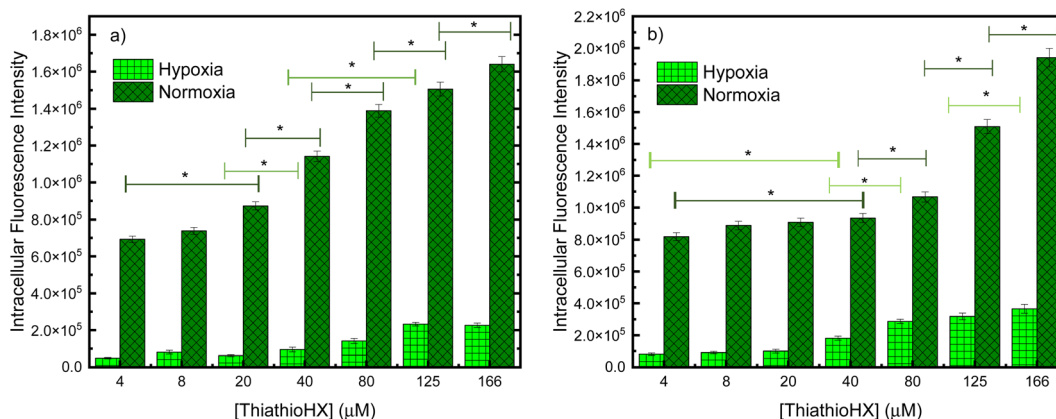
Fig. 8 Intracellular fluorescent intensities of ROS sensor DCF-DA in (a) B16F10 cells and (b) HeLa cells. The increase in intracellular ROS generation in cells treated with UVA and ThiathioHX was calculated relative to the control where the cells were treated with 5 \text{J cm}^{-2} of UVA but with no ThiathioHX. * denotes p < 0.05 .
