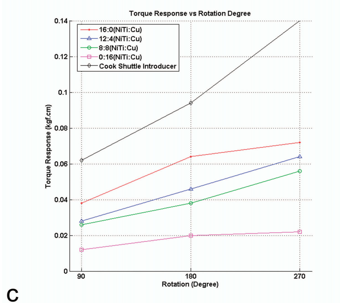
Figure 3 Torque transmission test fixture setup and test result. (a) The distal shaft is fixed to a freely-rotating collet (arrow) that indicates the angular response to torque. (b) A meter on the proximal shaft recorded transmitted torque after 90–270° tip rotation. (c) Comparative torquability values for different braiding layer configurations. Higher torque response values indicate greater torquability.
