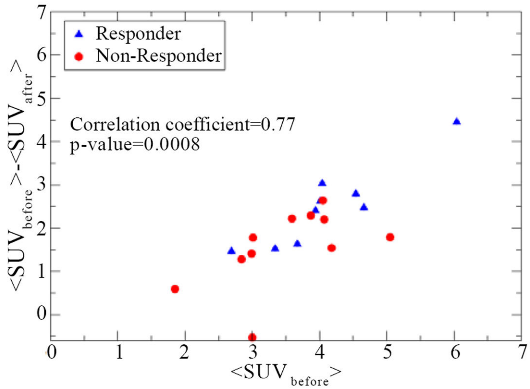
Figure 4. Scatter plot of the difference \langle \text{SUV}_{\text{before}} \rangle - \langle \text{SUV}_{\text{after}} \rangle as a function of \langle \text{SUV}_{\text{before}} \rangle . A significant correlation is seen among those quantities.
