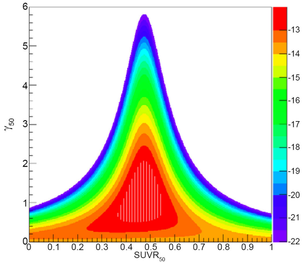
Figure 2. Two-dimensional plot of the log-likelihood as a function of SUVR_{R50} and \gamma_{50} . The most likely parameters are defined by the maximum log-likelihood.
