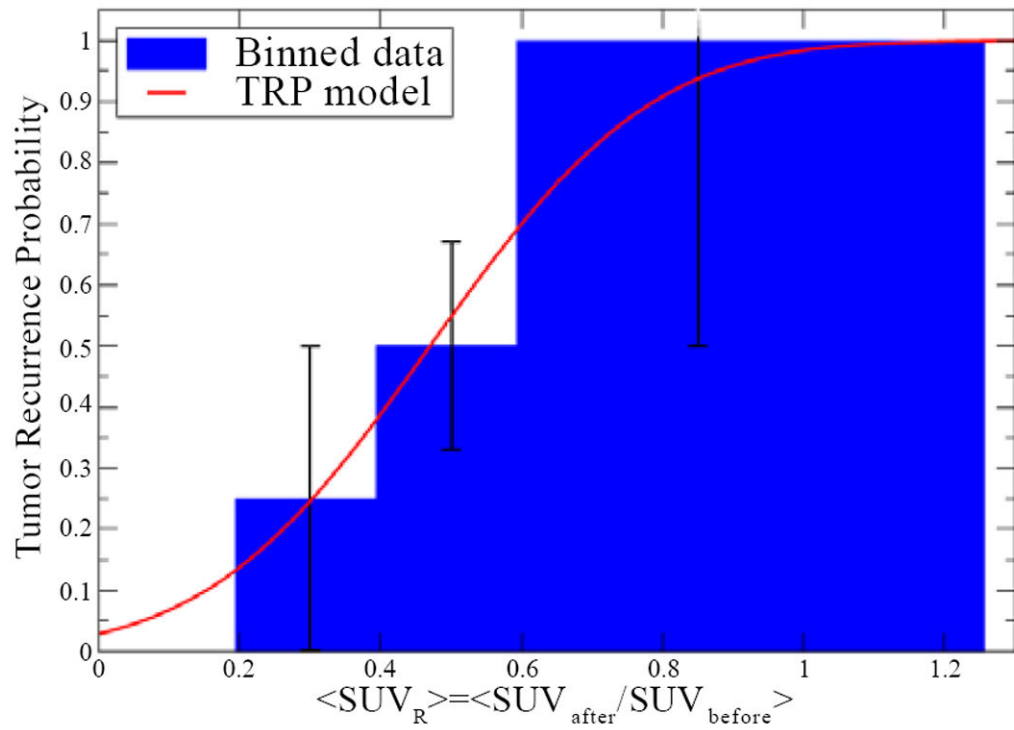
Figure 3. Tumor recurrence probability model compared to data represented in a histogram with 3 bins. The model reasonably represents the data despite large error bars resulting from the small patient sample.
