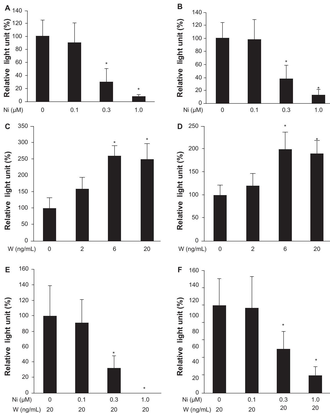
Figure 4 Luciferase assay. A luciferase assay was performed with TOPflash after the addition of Wnt3a or niclosamide to Huh-6 cells ( A , C , and E ) and Hep3B cells ( B , D , and F ). Luciferase activity of TOPflash was calculated as relative light units divided by that of pRL-TK. Wnt3a increased the luciferase activity of TOPflash ( C and D ). Luciferase activity was suppressed by niclosamide with ( E and F ) or without ( A and B ) Wnt3a (2 ng/mL).
