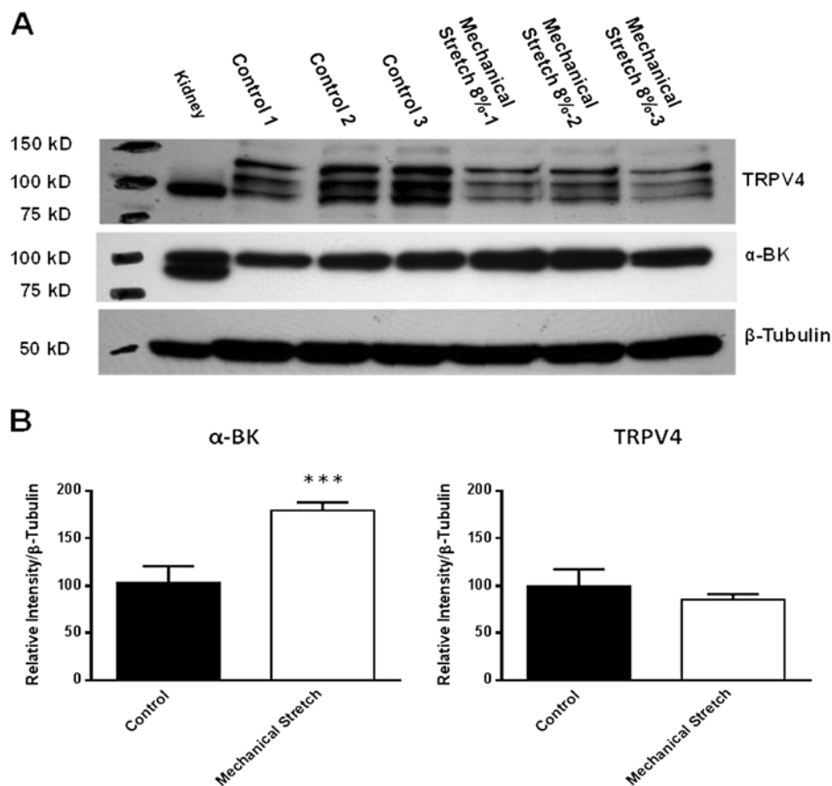
Figure 1 The effects of mechanical stretch on α-BK and TRPV4 protein levels in chondrocytes. (A) Expression of α-BK and TRPV4 channels in equine articular chondrocytes following exposure to mechanical stretch for 8 h. (B) The fold increase in the expression of α-BK and TRPV4 channels based on densitometric analysis of western blot by comparing to a housekeeping protein (β-tubulin). Data presented the mean ± S.E. and statistical significance is indicated by *** = P < 0.001 compared to unstretched controls.
