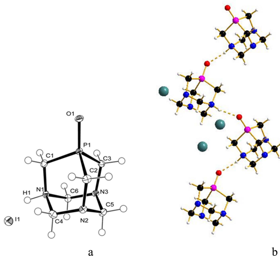
Fig. 4 (a) Molecular structure (ORTEP diagram) of [PTA(O)-H]·[I] ( 4 ) showing the atom labelling scheme. (b) 1D hydrogen bond of [PTA(O)-H] + chain. Hydrogen bonding interactions are highlighted as dashed lines. Color code: C, black; H, white; O, red; N, blue; P, purple; I, dark green. Thermal ellipsoids are shown at a 50% probability level. Selected bond lengths (Å) and angles (°): P1–C1 1.8175(13); P1–C2 1.8184(14); P1–C3 1.8160(14); P1–O1 1.4931(10); N1–C1 1.5005(17); N1–C4 1.5233(17); N1–C6 1.5288(17); N1–H1 0.897(18); N2–C4 1.4393(17); N2–C5 1.4719(17); N2–C2 1.4841(18); N3–C6 1.4390(17); N3–C5 1.4710(17); N3–C3 1.4864(17); O1–P1–C1 112.40(6); O1–P1–C3 119.29(6); C1–P1–C3 100.60(6); O1–P1–C2 118.37(6); C1–P1–C2 100.61(6); C3–P1–C2 102.62(6); C1–N1–C4 110.92(10); C1–N1–C6 110.72(10); C4–N1–C6 108.66(10); C4–N2–C5 109.69(10); C4–N2–C2 112.59(11); C5–N2–C2 112.47(11); C6–N3–C5 110.14(11); C6–N3–C3 113.43(10); C5–N3–C3 111.81(10); N1–C1–P1 109.83(8); N2–C2–P1 108.35(9); N3–C3–P1 108.33(9).
