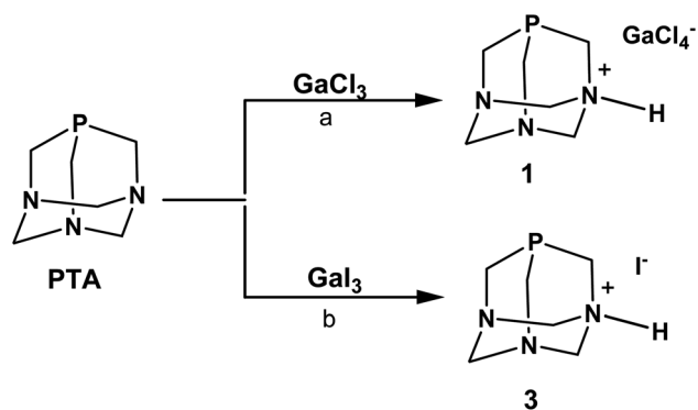
Scheme 1 Products of reactions of PTA with GaCl 3 and GaI 3 . Reaction conditions: (a) [Ga]:[P] = 1:1.2; DCM@r.t. or DCM@0 °C; or DCM/Et 3 N@r.t. (b) [Ga]:[P] = 1:1.2; EtOAc@r.t. or Et 2 O@r.t. or solid state reaction.
