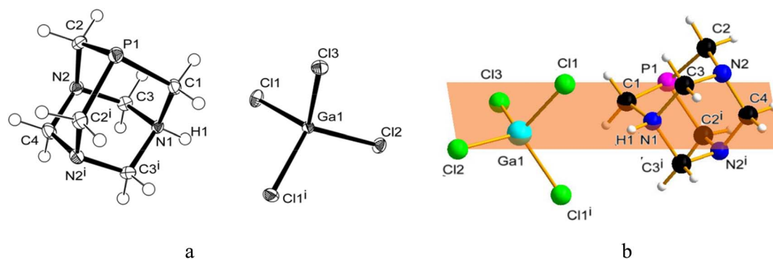
Fig. 2 (a) Molecular structure (ORTEP diagram) of [PTA-H] + [GaCl 4 ] - (1) showing the atom labelling scheme. Thermal ellipsoids are shown at a 50% probability level. (b) Molecular structure highlighting the mirror plane. Color code: C, black; H, white; N, blue; P, purple; Cl, green; Ga, light blue selected bond lengths (Å) and angles (°): P1–C1 1.854(3); P1–C2 1.8566(19); N1–C1 1.511(3); N1–C3 1.531(2); N2–C2 1.472(2); N2–C3 1.436(2); N2–C4 1.467(2); Ga1–Cl1 2.1862(5); Ga1–Cl2 2.1582(6); Ga1–Cl3 2.1737(6); C1–P1–C2 96.58(8); C2–P1–C2#1 96.68(12); C1–N1–C3 111.81(12); C3–N1–C3#1 108.64(18); C3–N2–C4 109.88(15); C2–N2–C3 112.13(14); C2–N2–C4 111.57(16); N2–C2–P1 113.85(12). Symmetry transformations used to generate equivalent atoms: x , – y + 1/2, z .
